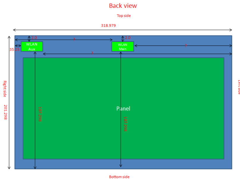
Fig.10 Antenna position of EUT (Back view)
