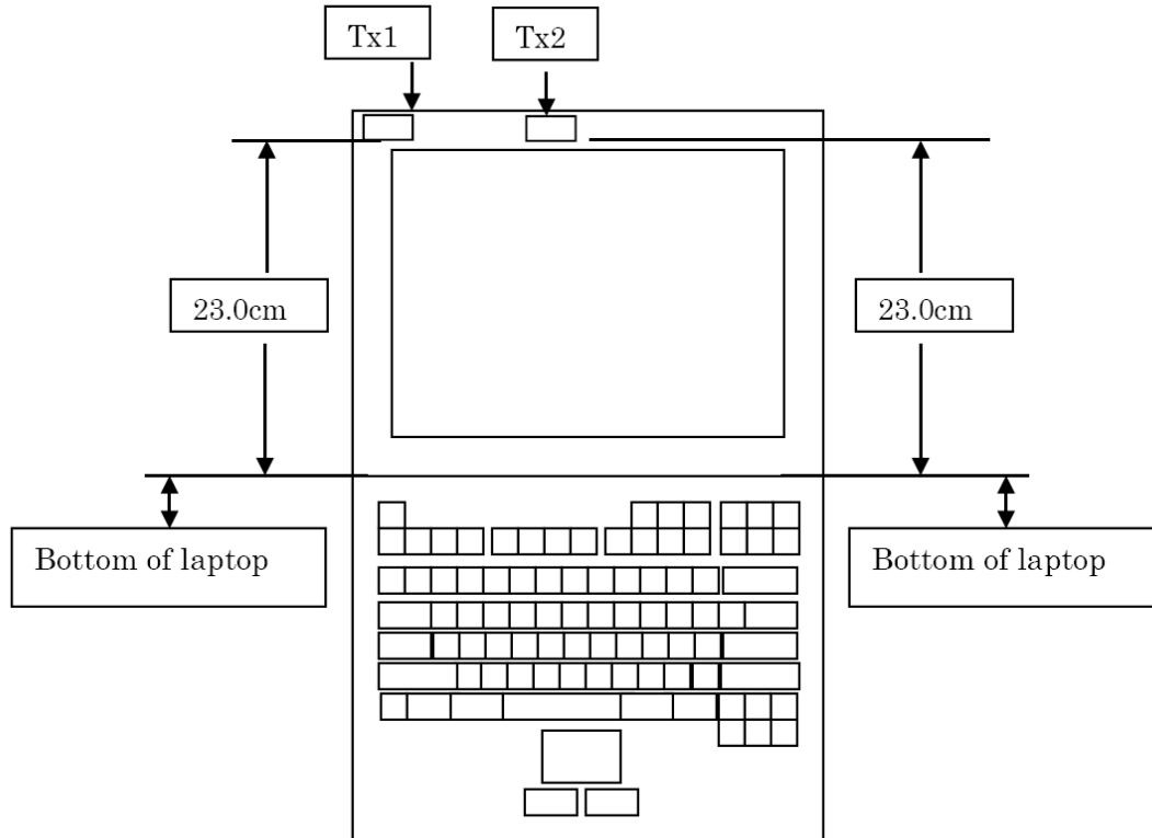
Diagram Showing WLAN Antenna Positions
