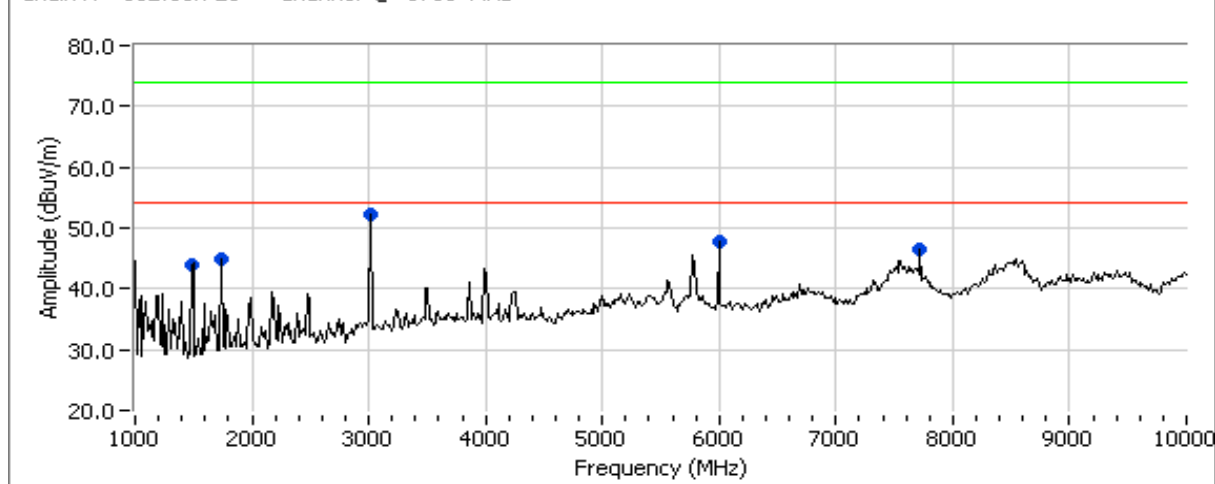
Chain A 802.11n-20 Channel @ 5785 MHz
