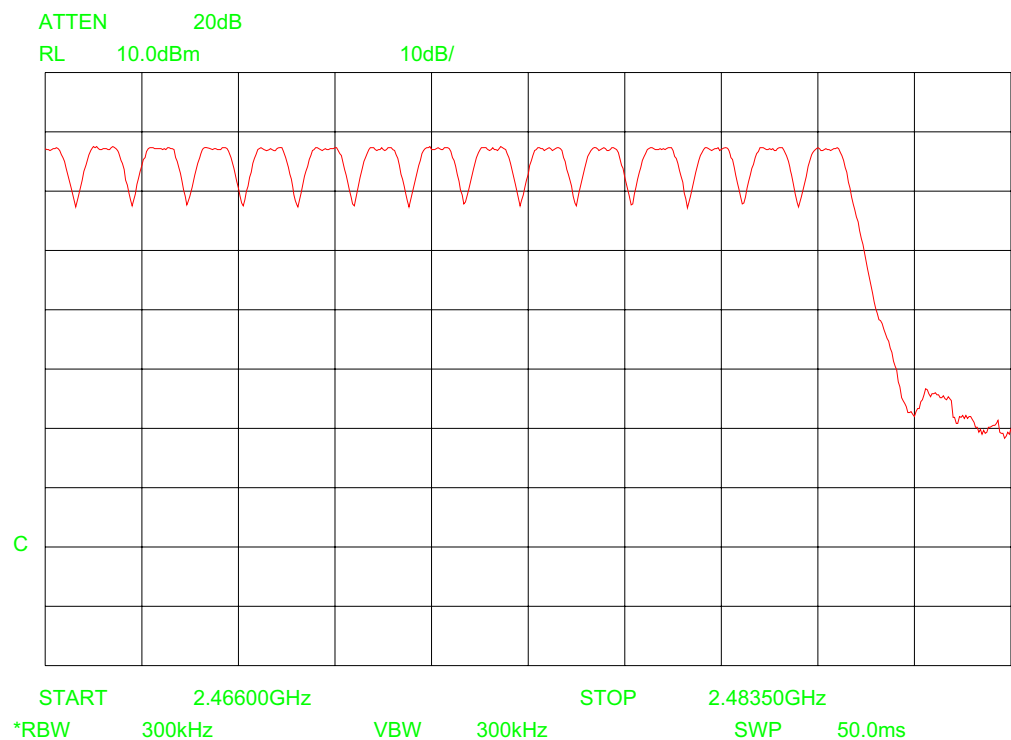
Plot 7 – Number of channels (channels 65-79, GFSK mode)
