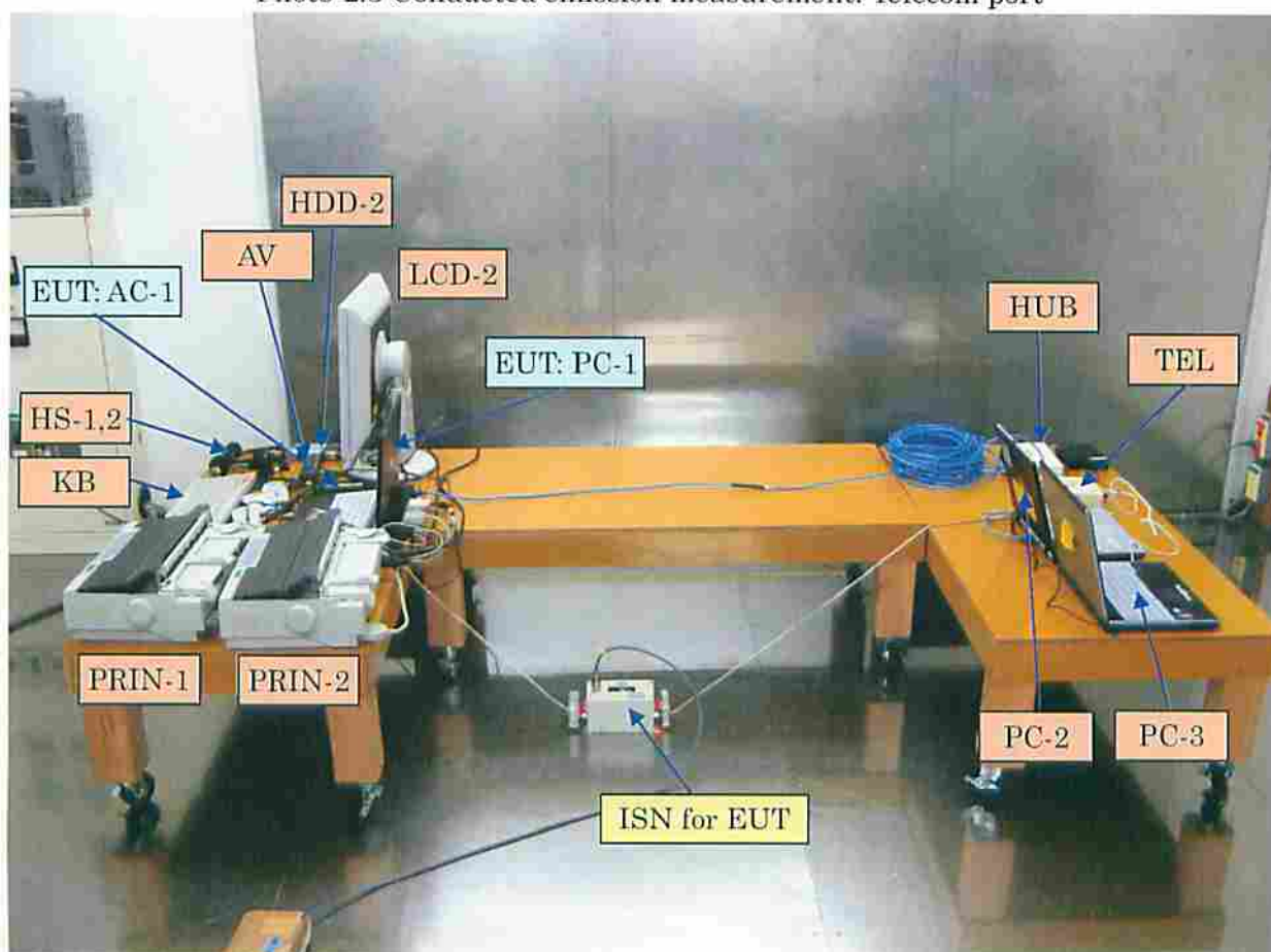
Photo-2.3 Conducted emission measurement: Telecom port
