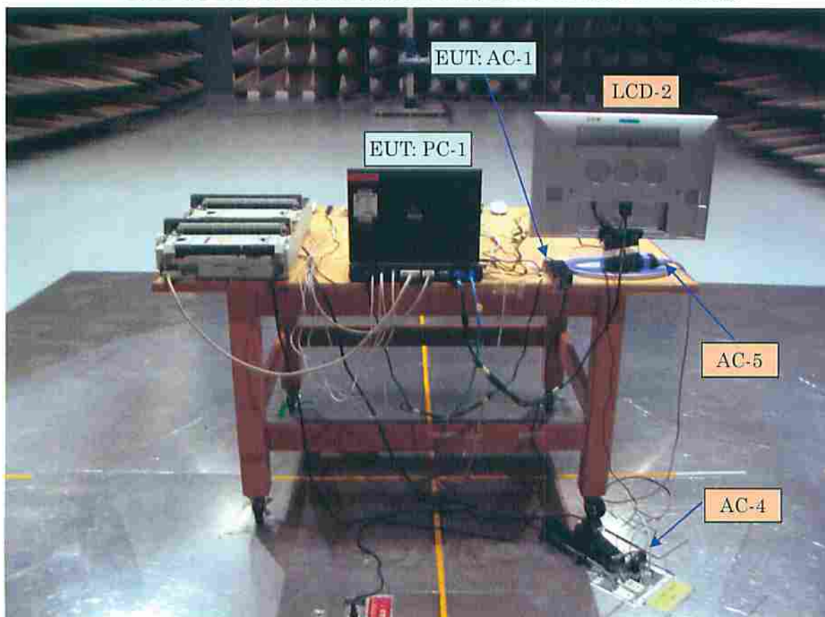
Photo-1.2 Radiated emission measurement for 30-1000 MHz (Back)
