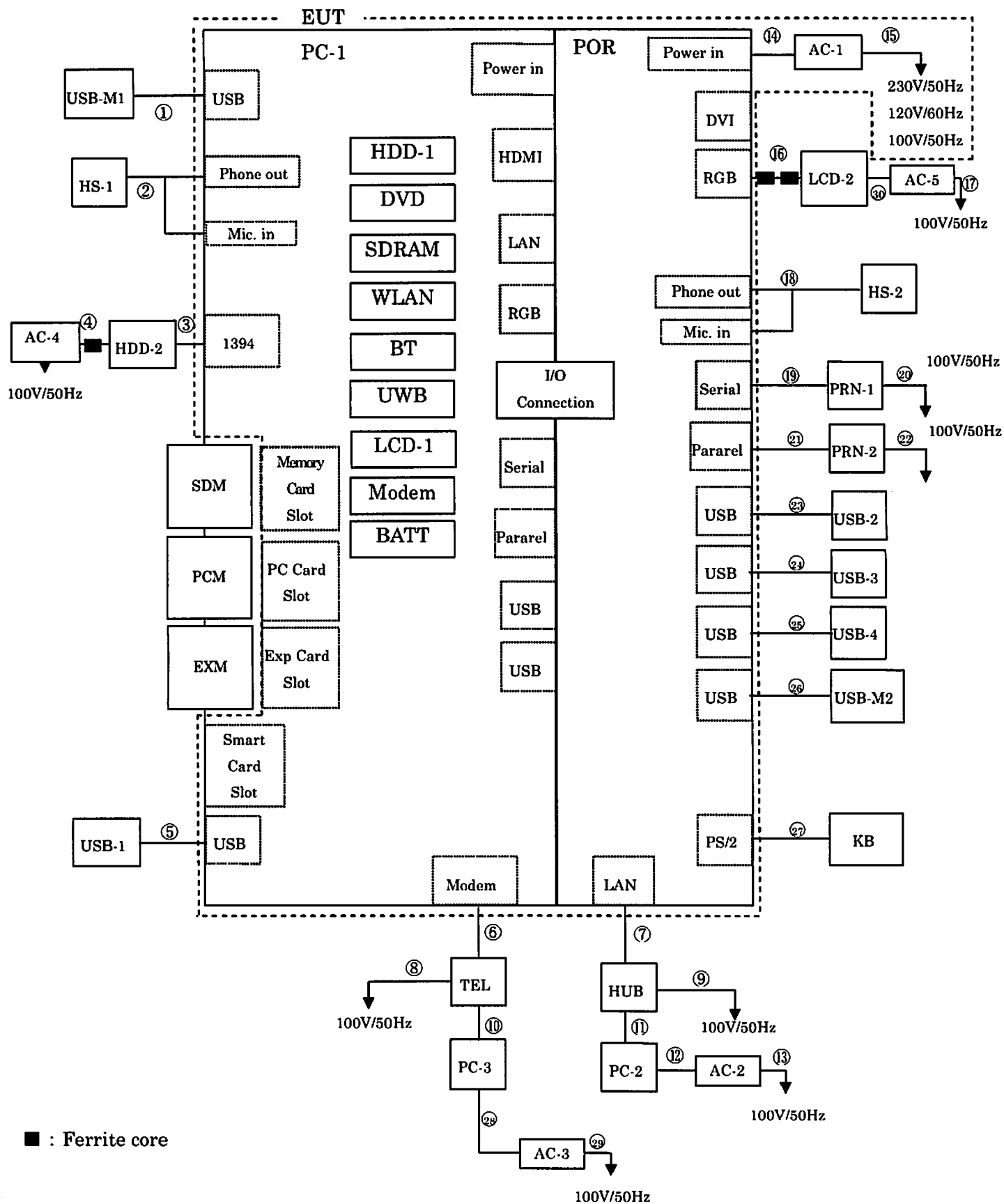
Figure-1 System configuration and cables
