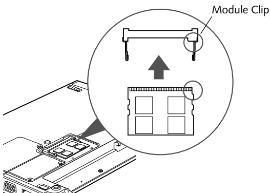
Figure 4-13. Aligning the memory module
