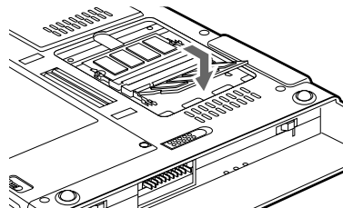
Figure 2-9. Installing a DIMM Module
