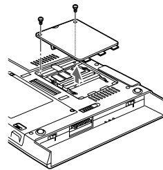
Figure 2-8. Accessing the Memory Slot
