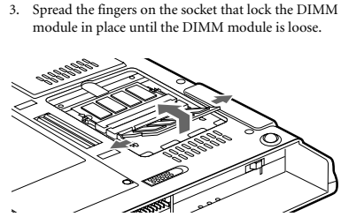
Figure 2-10. Removing a DIMM Module
