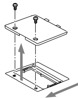
Figure 4-2. Opening the Memory Upgrade Compartment
