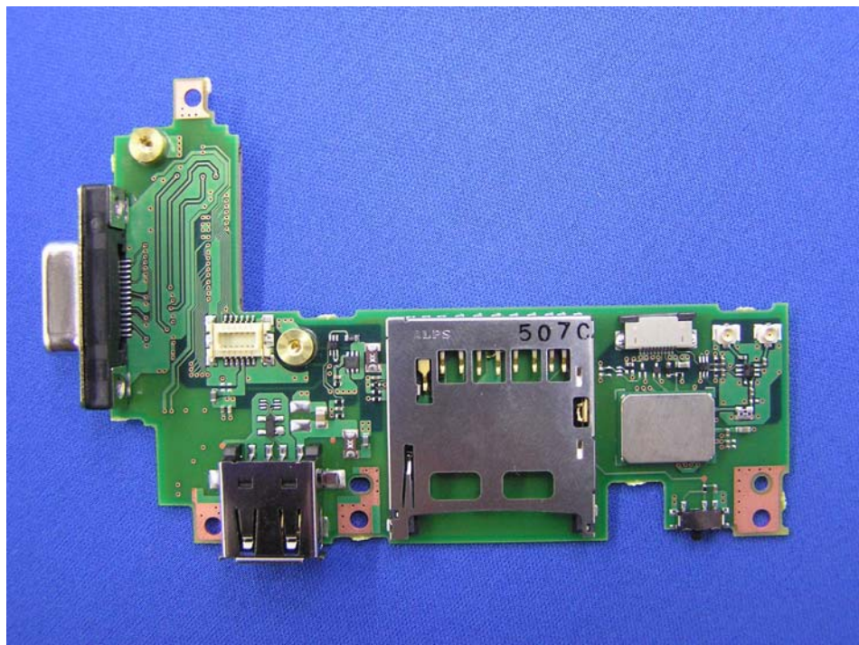
Circuit Board with Bluetooth Module(Top)
