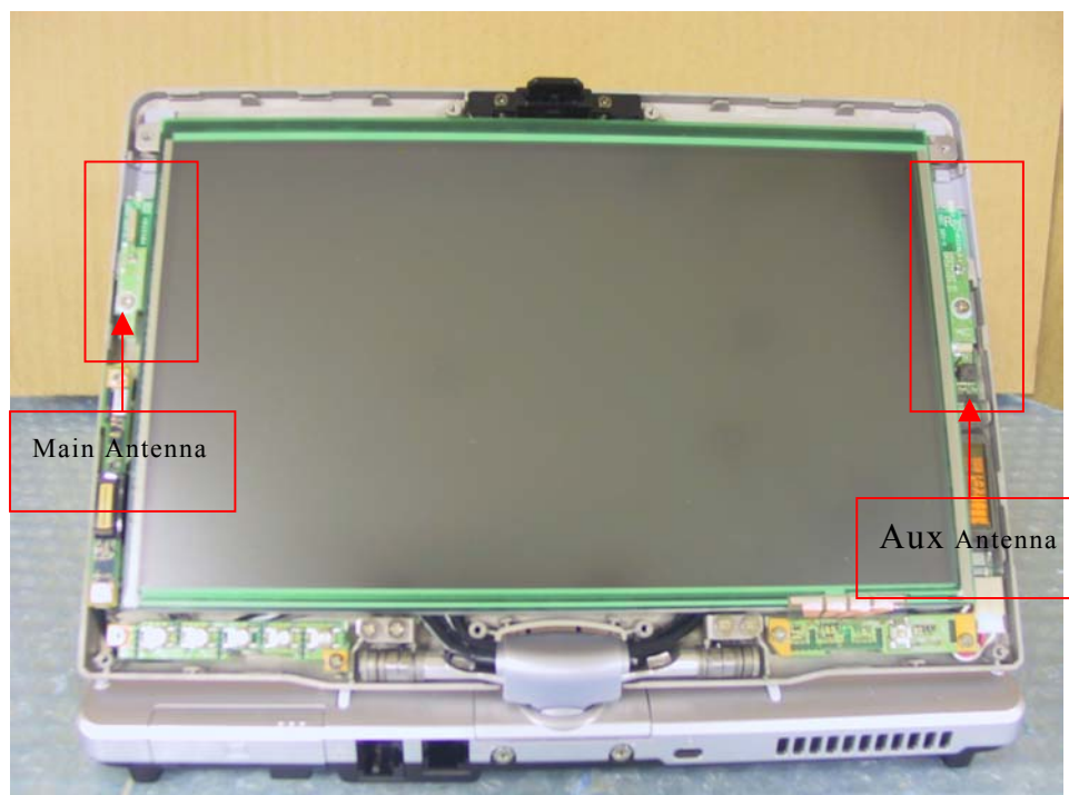
Front Panel (Cover off)
