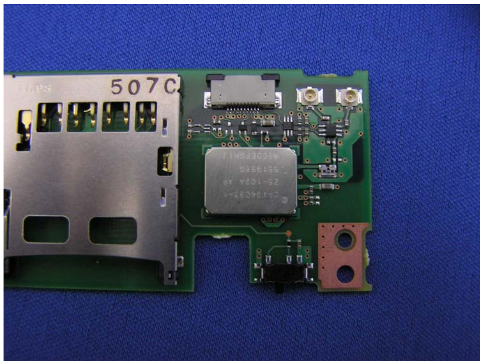
Bluetooth Module (with Shield)
