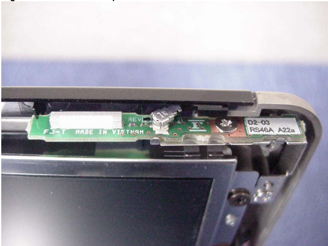
Right Antenna Location - exploded view
