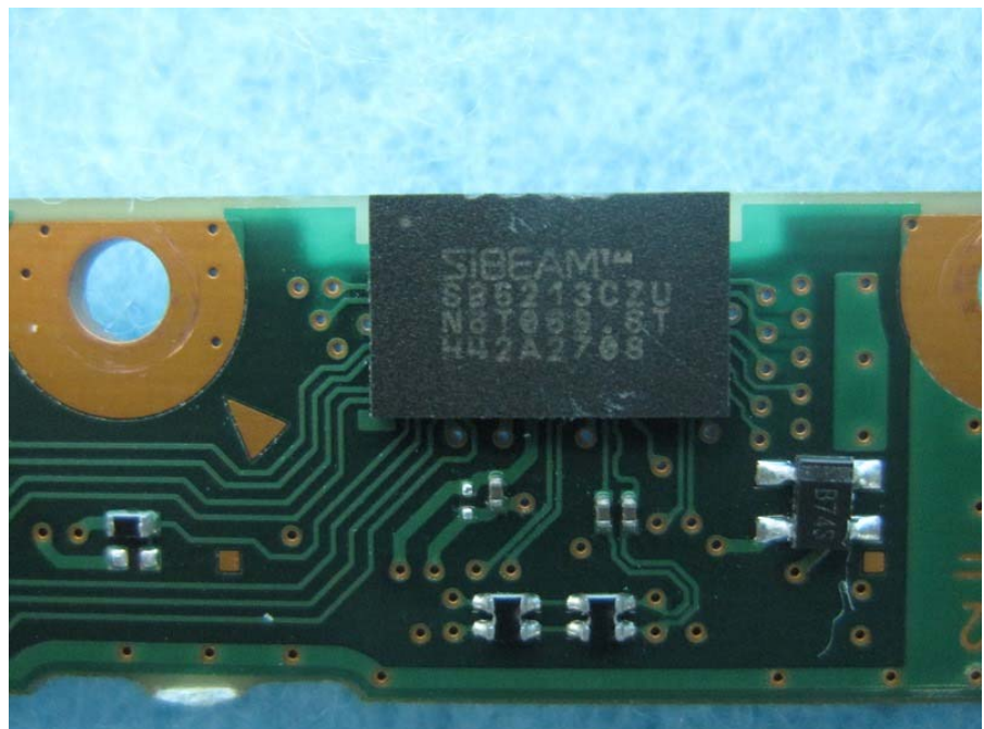
60G Module and antenna Model No.: SB6213
