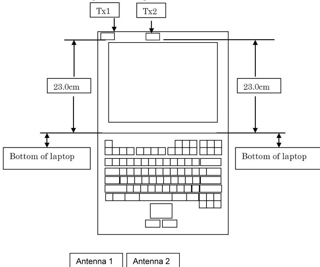
Diagram Showing WLAN Antenna Positions
