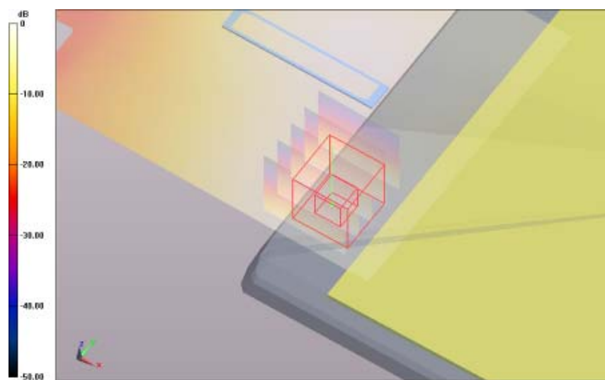
SAR Measurement Plot 134
