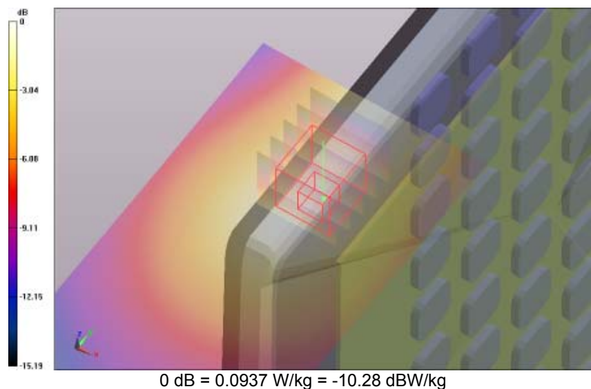
SAR Measurement Plot 122
