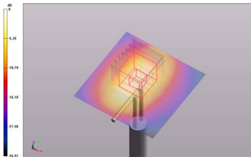
SAR Measurement Plot 158
