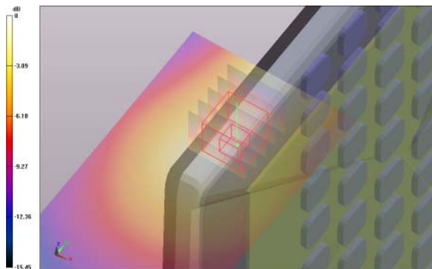
SAR Measurement Plot 123
