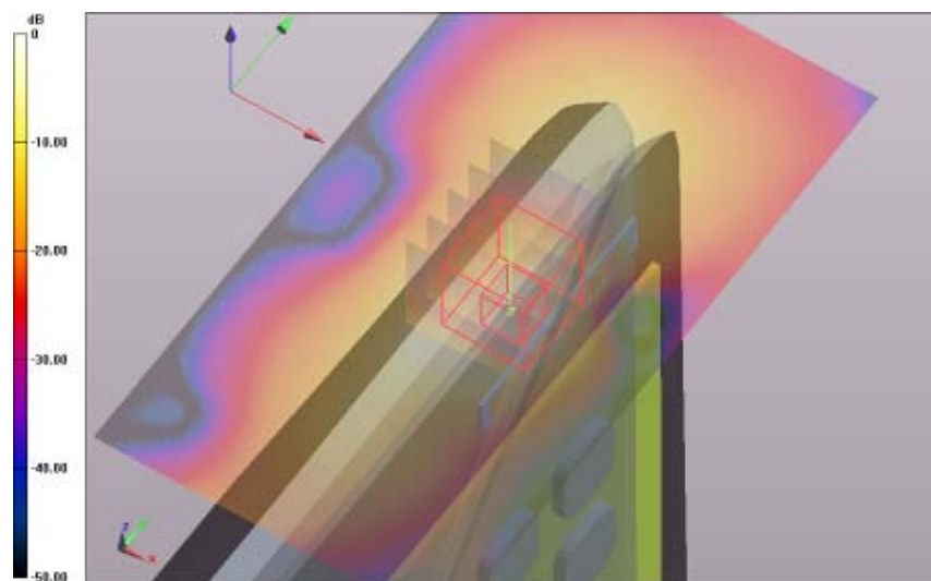
SAR Measurement Plot 175
