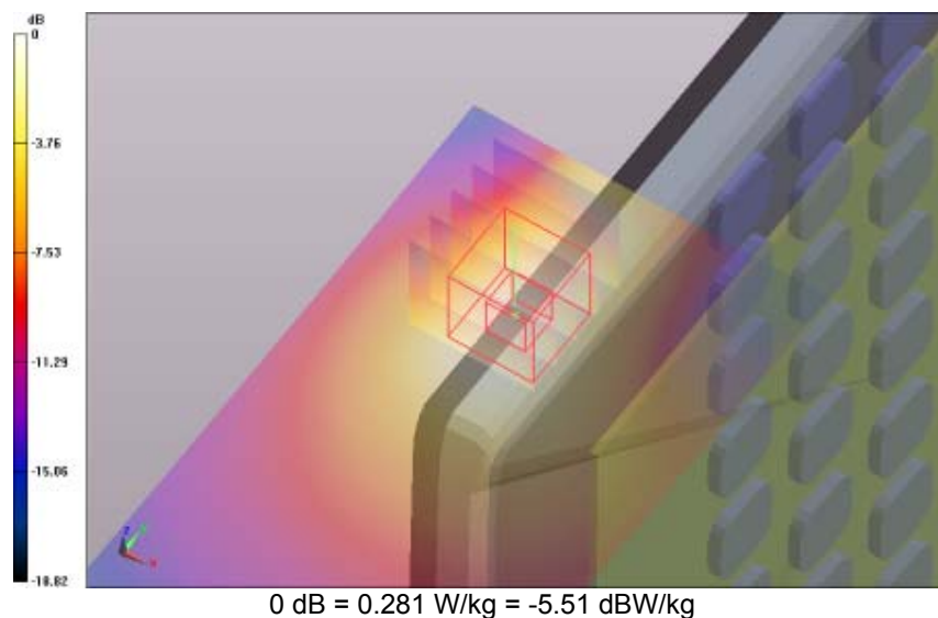
SAR Measurement Plot 182
