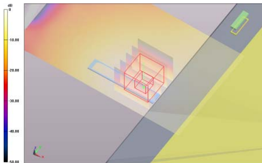
SAR Measurement Plot 162
