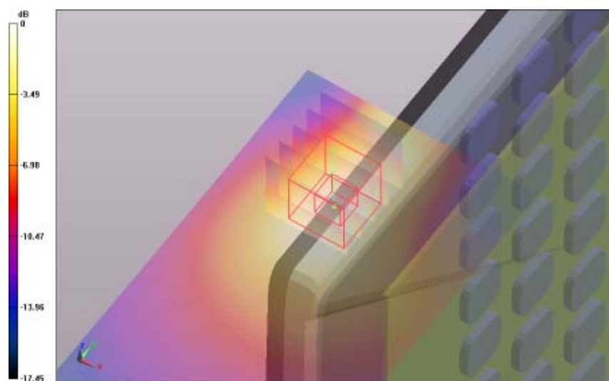
SAR Measurement Plot 180
