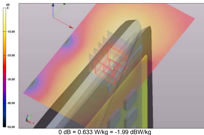
SAR Measurement Plot 146
