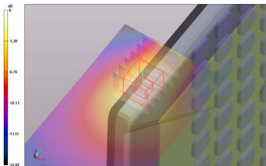
SAR Measurement Plot 97
