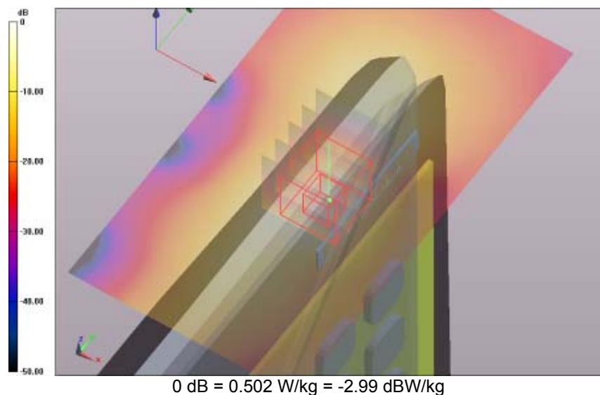
SAR Measurement Plot 151
