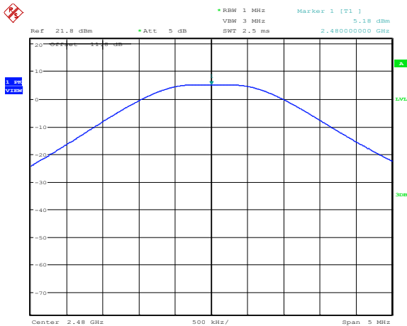
Figure 8.6-3: Output power on high channel
