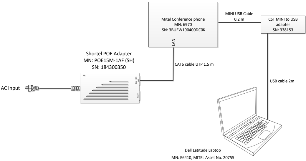
Figure 3.6-1: Setup diagram
