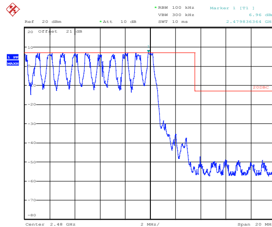
Figure 8.6-33: Conducted spurious emissions band edge for BT, hopping sequence is on
