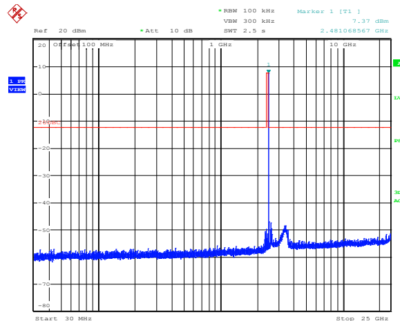
Figure 8.6-52: Conducted spurious emissions for BLE, high channel
