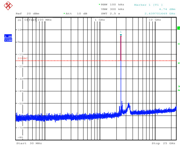
Figure 8.6-51: Conducted spurious emissions for BLE, mid channel
