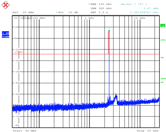
Figure 8.6-29: Conducted spurious emissions for BT, high channel
