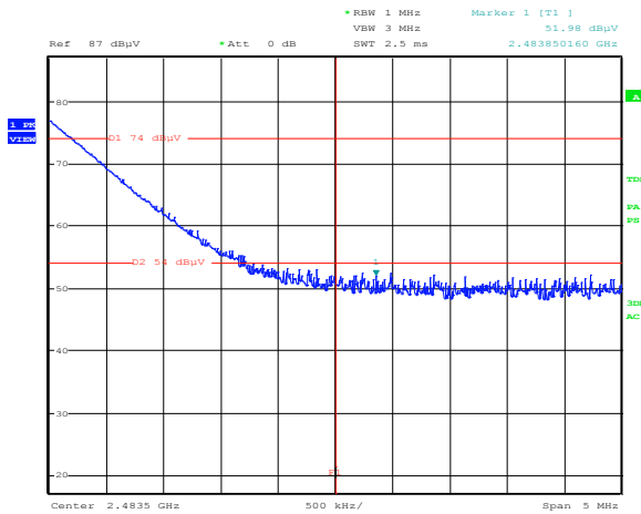
Figure 8.6-56: Radiated spurious emissions Upper band edge emission for BLE, High channel. F1 = 2.4835 GHz (beginning of restricted band)
