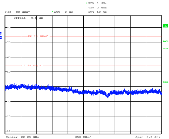
Figure 8.6-45: Radiated spurious emissions for BT, mid channel, 18 to 26.5 GHz
