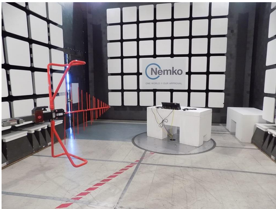
Figure 8.6-69: Radiated spurious (out-of-band) emissions setup photo – 30 to 1000 MHz
