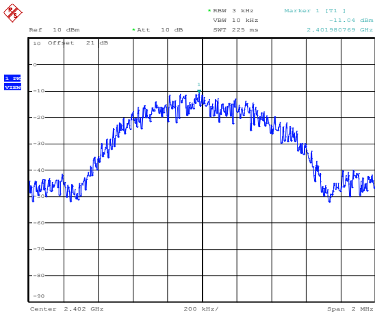
Figure 8.7-1: PSD sample plot on low channel
