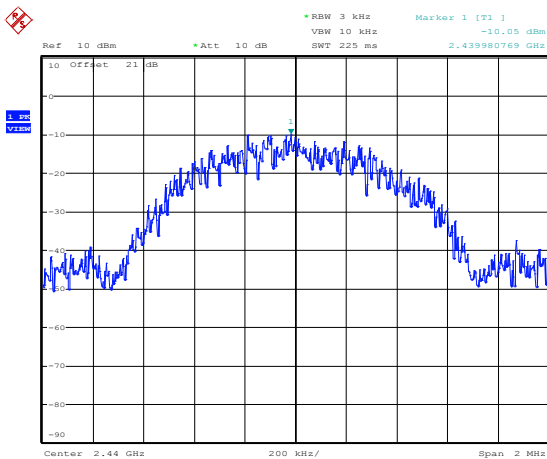
Figure 8.7-2: PSD sample plot on mid channel
