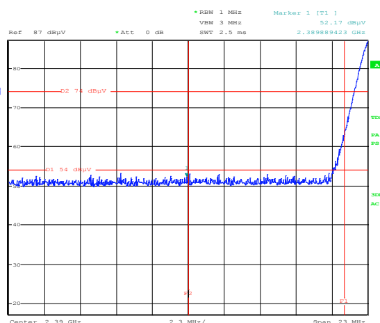
Figure 8.6-35: Radiated spurious emissions Lower band edge emission for BT, hopping is turned on. F_2 = 2.39 GHz (end of restricted band), F_1 = 2.4 GHz
