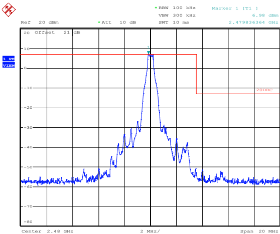
Figure 8.6-32: Conducted spurious emissions upper band edge for BT, high channel (hopping sequence is off)
