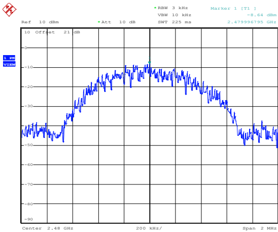
Figure 8.7-3: PSD sample plot on high channel
