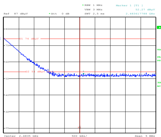
Figure 8.6-37: Radiated spurious emissions Upper band edge emission for BT, hopping is turned on. F1 = 2.4835 GHz (beginning of restricted band)
