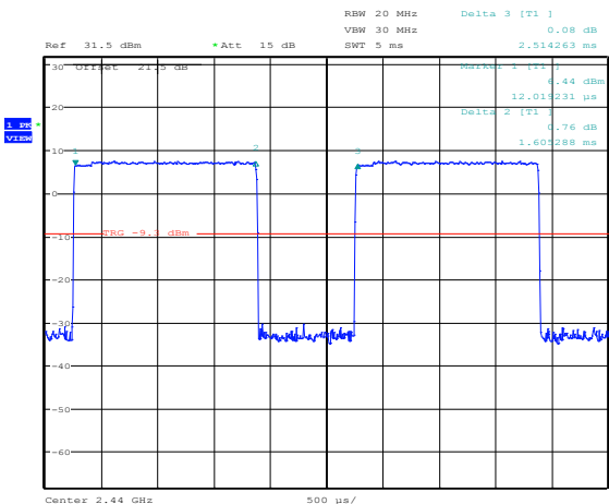
Figure 8.5-23: Pulse width for 2-EV3
