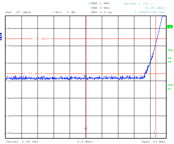
Figure 8.5-35: Radiated spurious emissions Lower band edge emission for BT, hopping is turned on. F2 = 2.39 GHz (end of restricted band), F1 = 2.4 GHz
