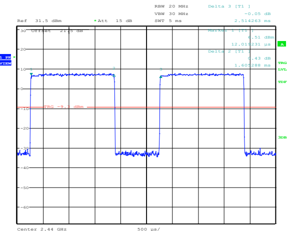
Figure 8.5-24: Pulse width for 3-EV3
