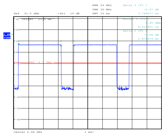
Figure 8.5-8: Pulse width for DH_3
