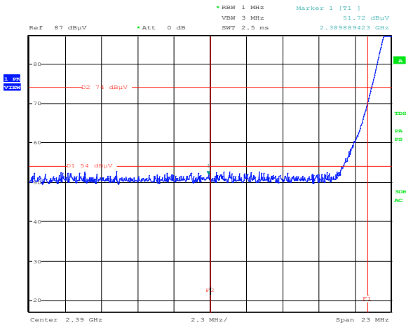
Figure 8.5-34: Radiated spurious emissions Lower band edge emission for BT, hopping is turned off – Low channel. F2 = 2.39 GHz (end of restricted band), F1 = 2.4 GHz
