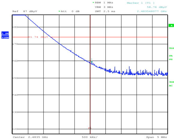
Figure 8.5-36: Radiated spurious emissions Upper band edge emission for BT, hopping is turned off – high channel. F1 = 2.4835 GHz (beginning of restricted band)
