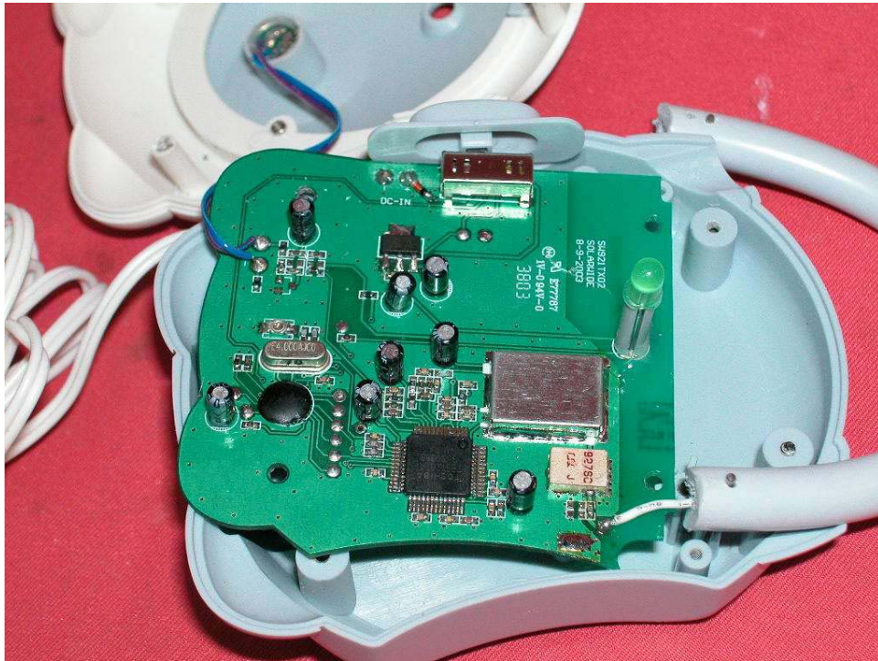
Main PCB comp side
