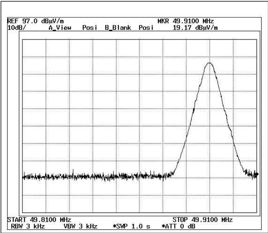
Un-modulated Carrier Channel B
