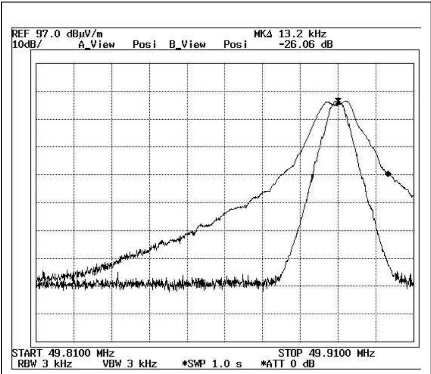
Modulated Carrier Channel B
