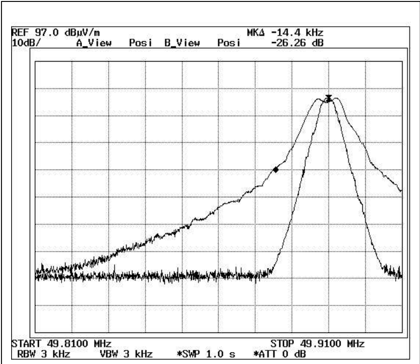
Modulated Carrier Channel B
