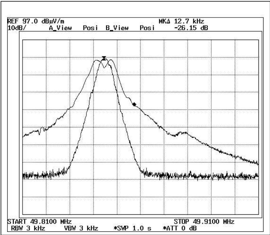
Modulated Carrier Channel A
