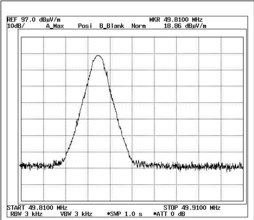
Un-modulated Carrier Channel A
