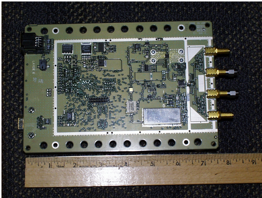
EUT (IM5) Board Bottom With VCO Shielding View
