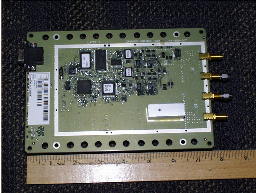
EUT (IM5) Board Top Without Shielding View
