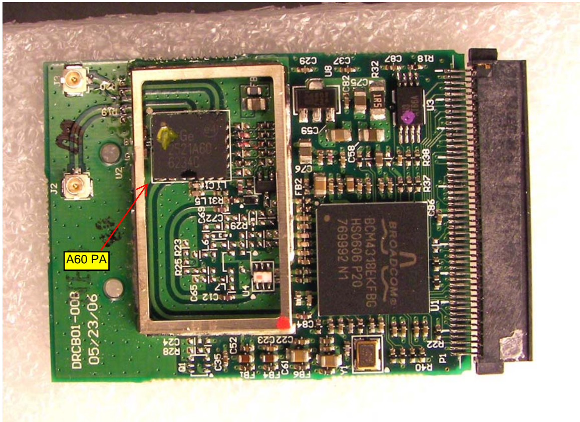
Close-up, showing A60 PA
