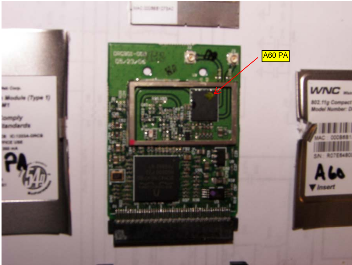
DRCB – Top View (shield removed) – showing new A60 PA
