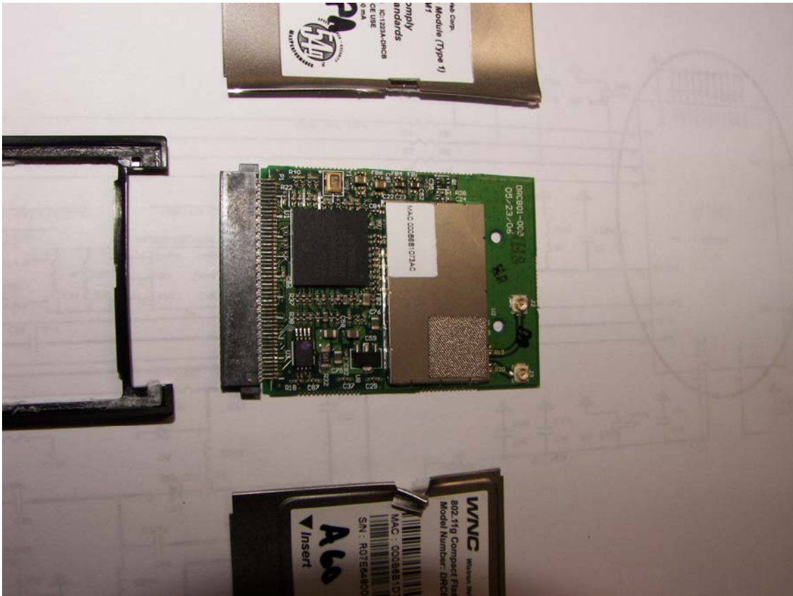
DRCB – Top View (Cover removed) – Close-up
