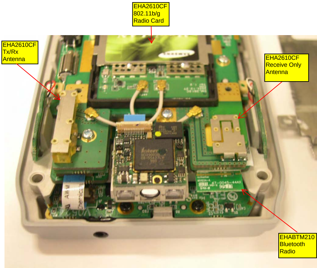
CN30 Radio/Antenna Placement
