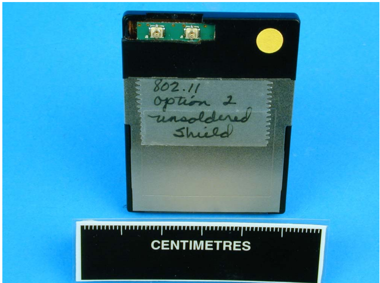
Top view of 802.11b Radio Module
