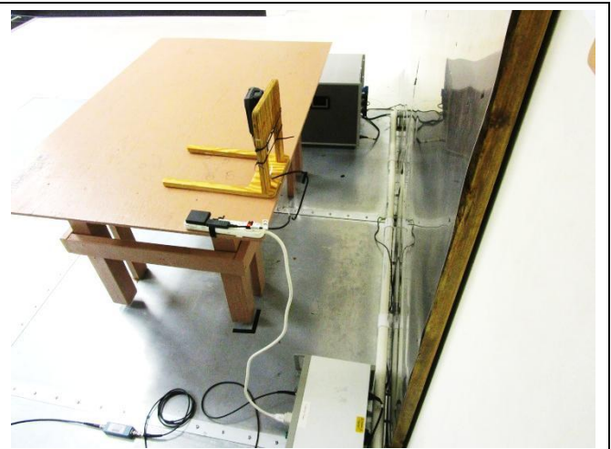
AC Conducted Emission (Rear View)
