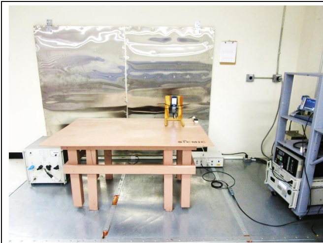
AC Conducted Emission (Front View)
