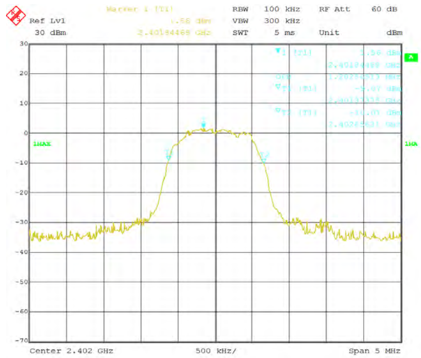
99% dB Bandwidth - Low Channel
