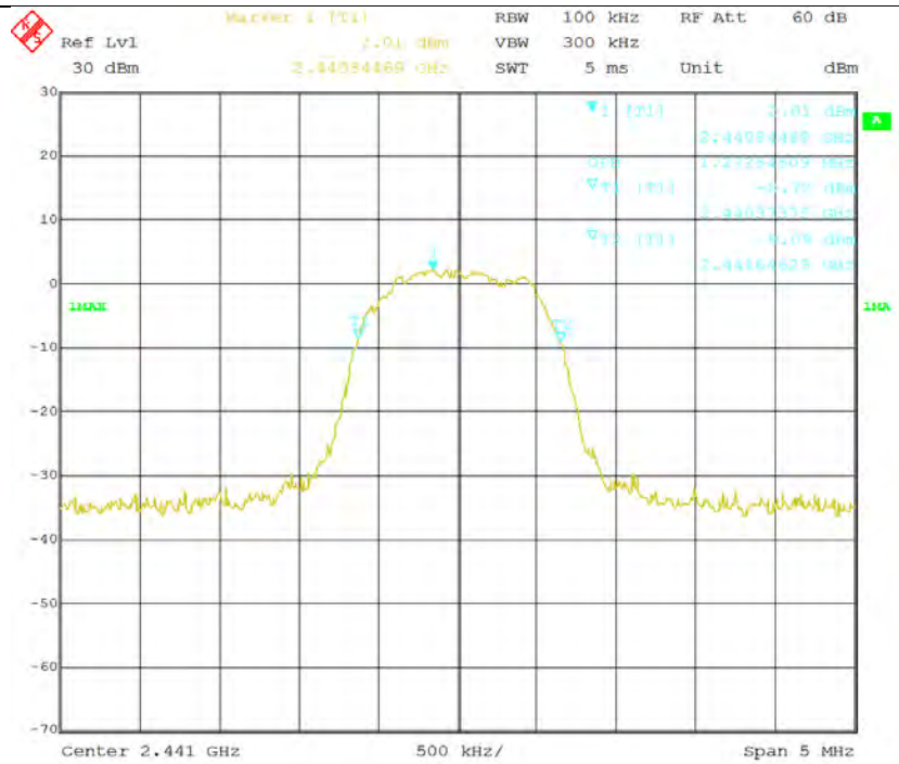
99% dB Bandwidth - Mid Channel
