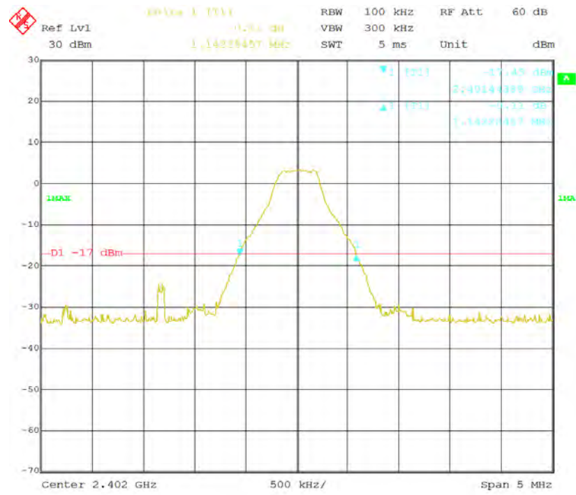
20dB Bandwidth - Low Channel (Basic Rate)
