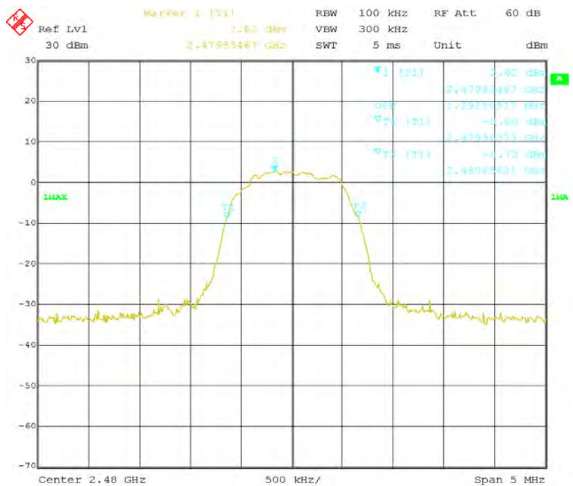
99% dB Bandwidth - High Channel
