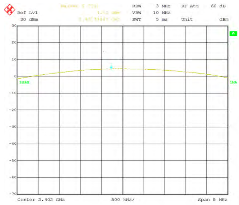
Output Power Low Channel (Bluetooth)
