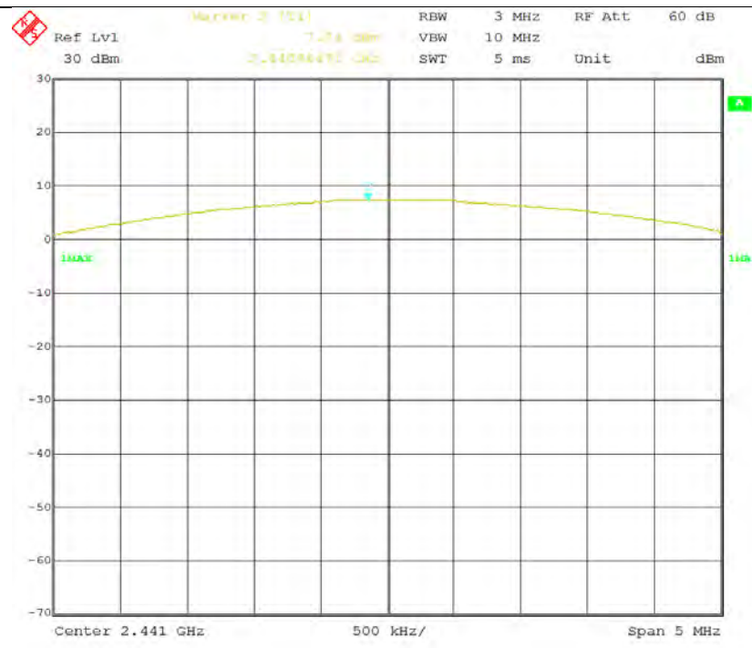
Output Power Mid Channel (Bluetooth)
