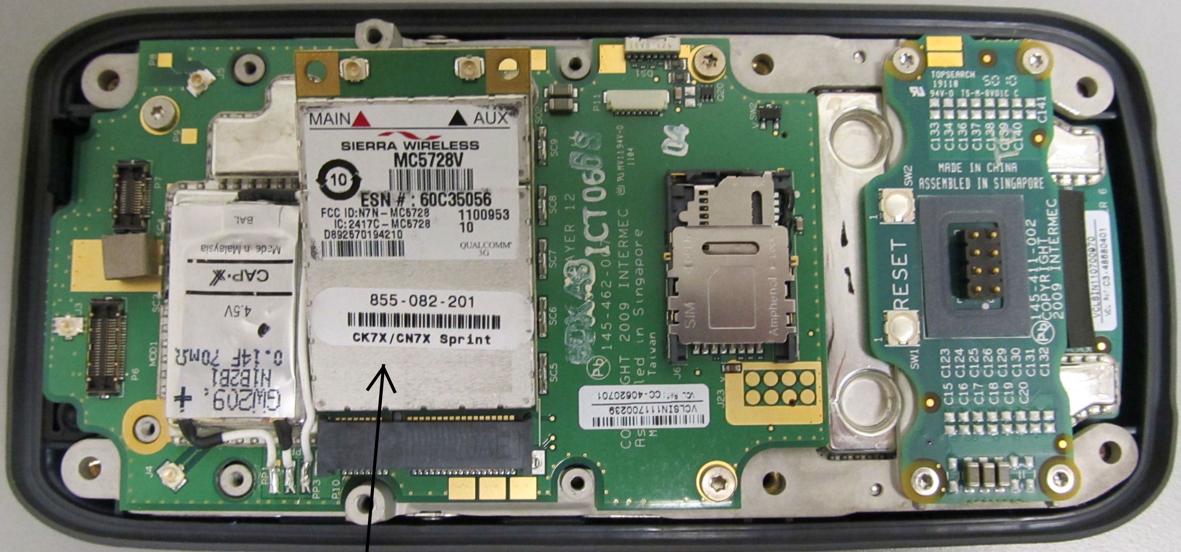
CDMA Radio
