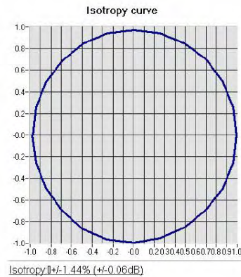
Isotropy at 1900 MHz
