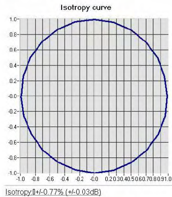
Isotropy at 835 MHz
