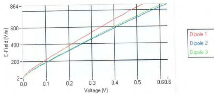
Calibration curves
