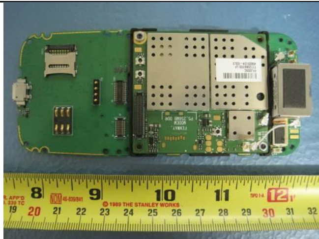
Internal PCBA Top View
