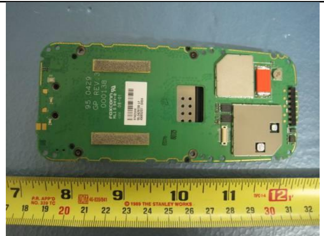
Internal PCBA Bottom View
