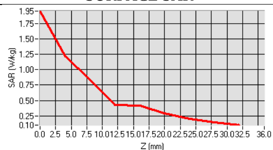
SURFACE SAR
