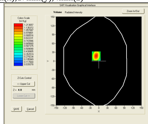
VOLUME SAR
