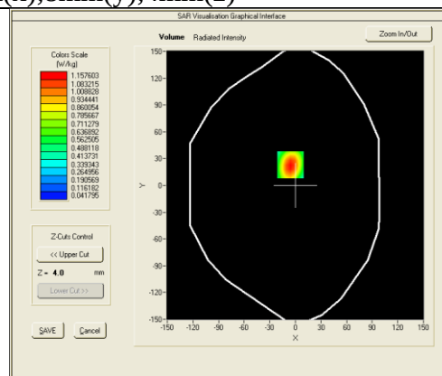
VOLUME SAR
