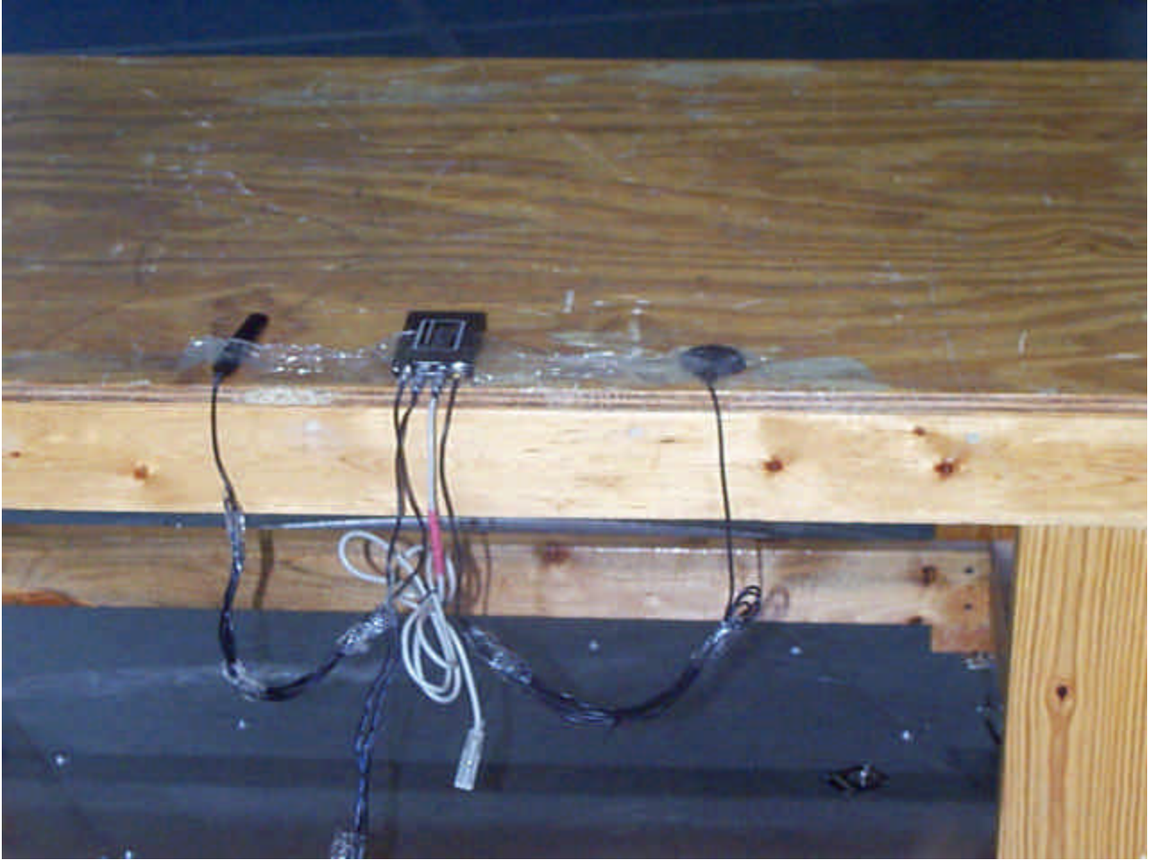
Figure 5 – Radiated Configuration 1
