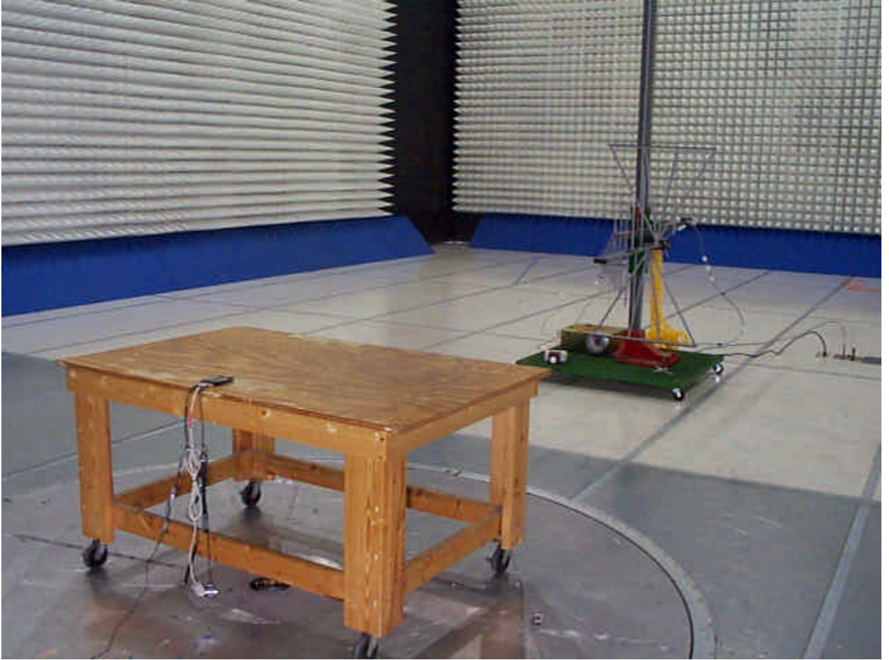
Figure 4 – Radiated Testing
