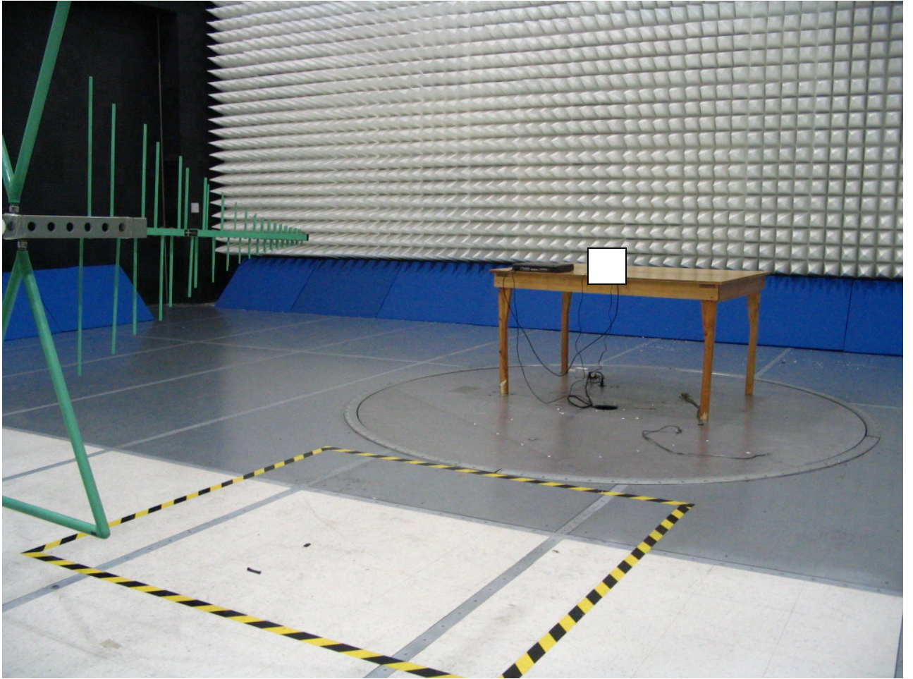
Figure 1: Radiated Emissions Testing
