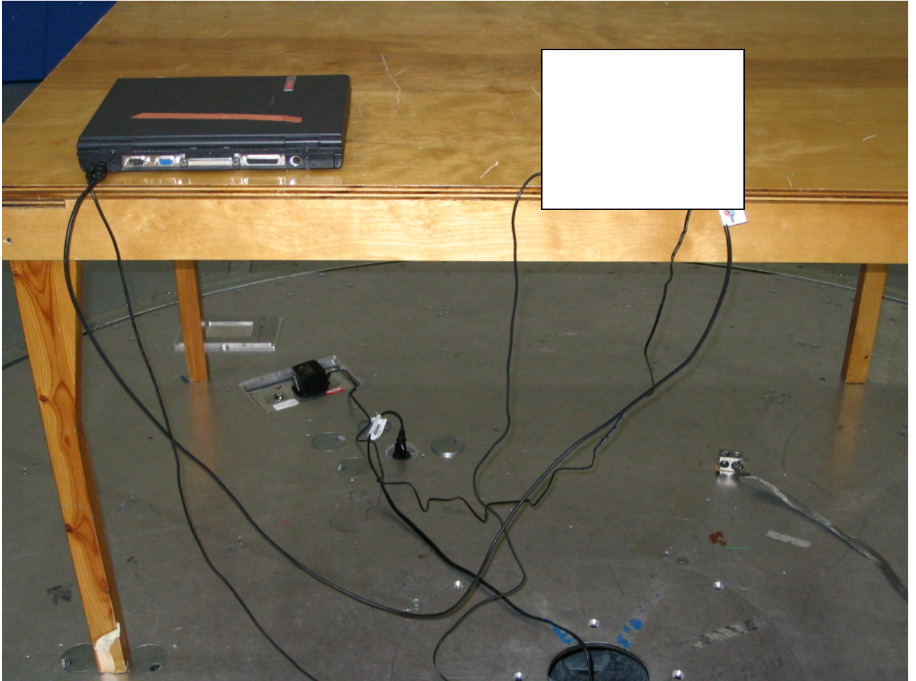
Figure 2: Radiated Emissions Testing
