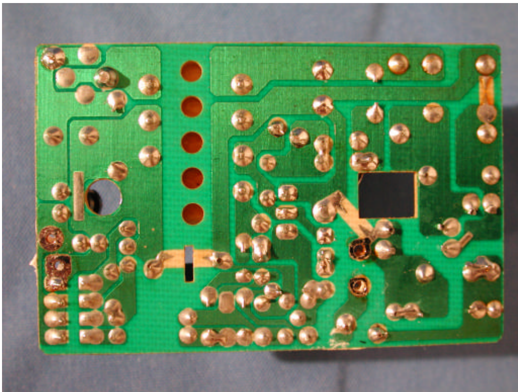
(28) EUT Photo
