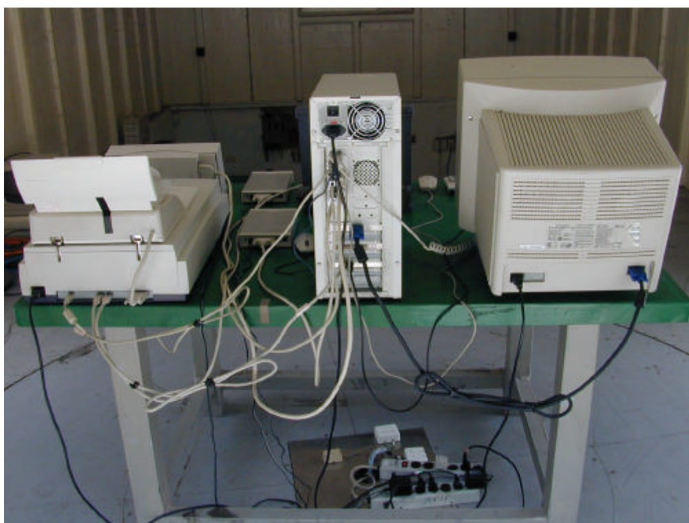
Back View of Radiated Test (Mode 1—Link PC, W/USB Cable (1.5M))
