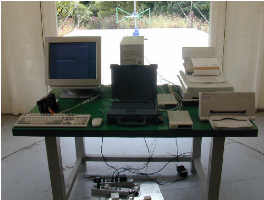
Back View of Radiated Test (Mode 2—Link PC, W/1394 Cable (1.5M))
