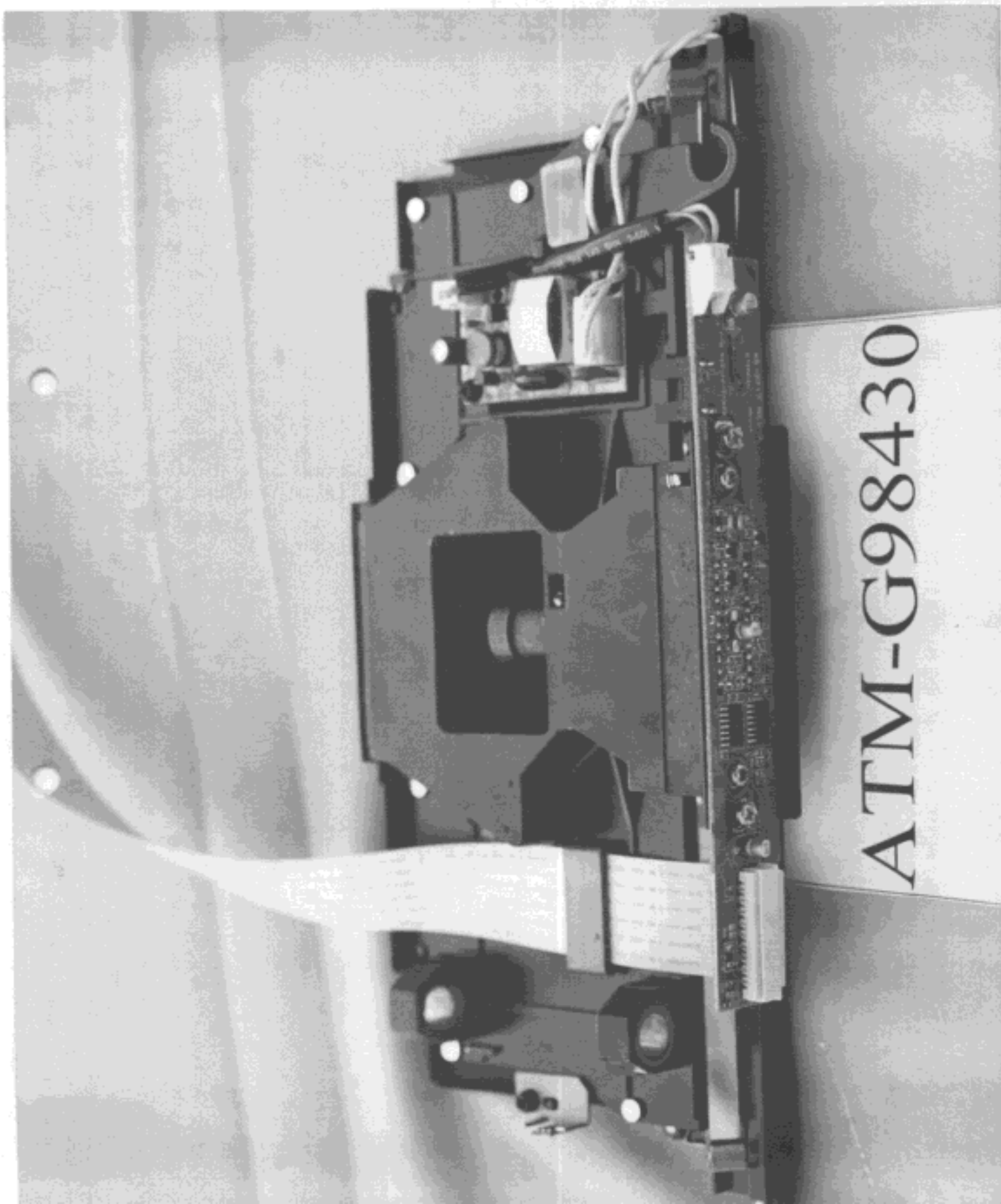
Figure 11 Back View of Scan Sensor Head
