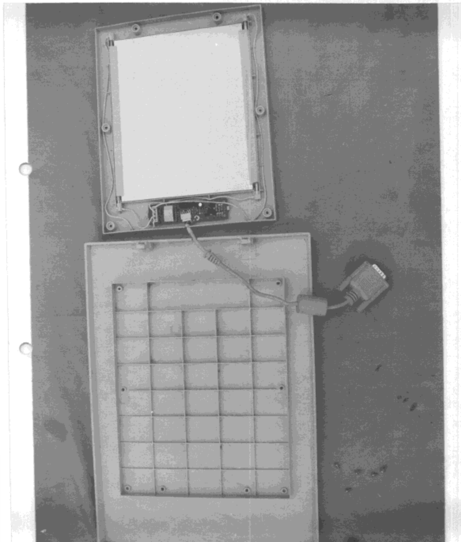
Figure 22 Top Cover, Internal View of Light Plate
