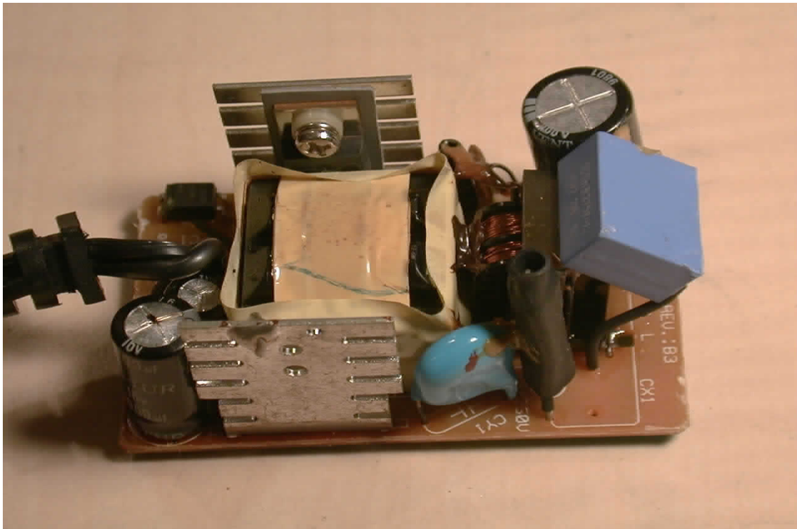
(32) EUT Photo (Mode 3:Bestec, BPA-201S-15)
