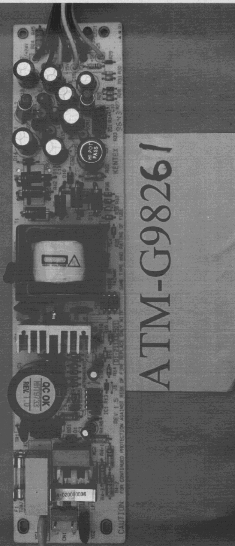
Figure 13 Switching Power Supply (Component Side)
