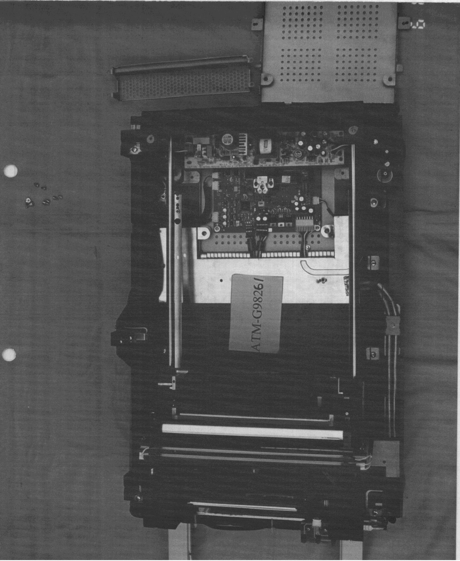
Figure 7 Metal Cover of Main Board and S.P.S Removed & Internal View
