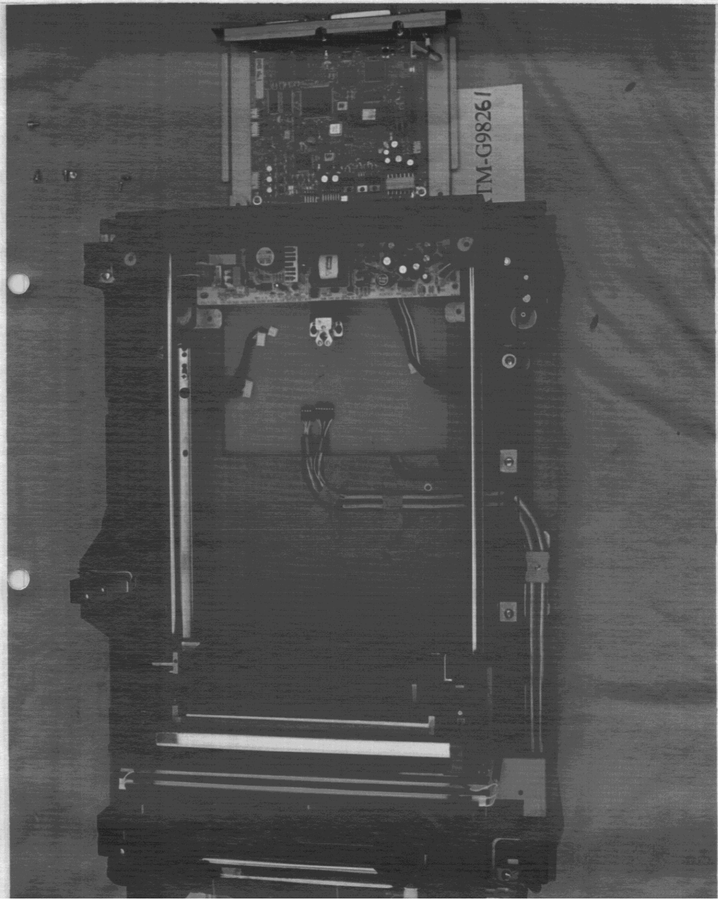
Figure 8 Removed Main Board & Internal View
