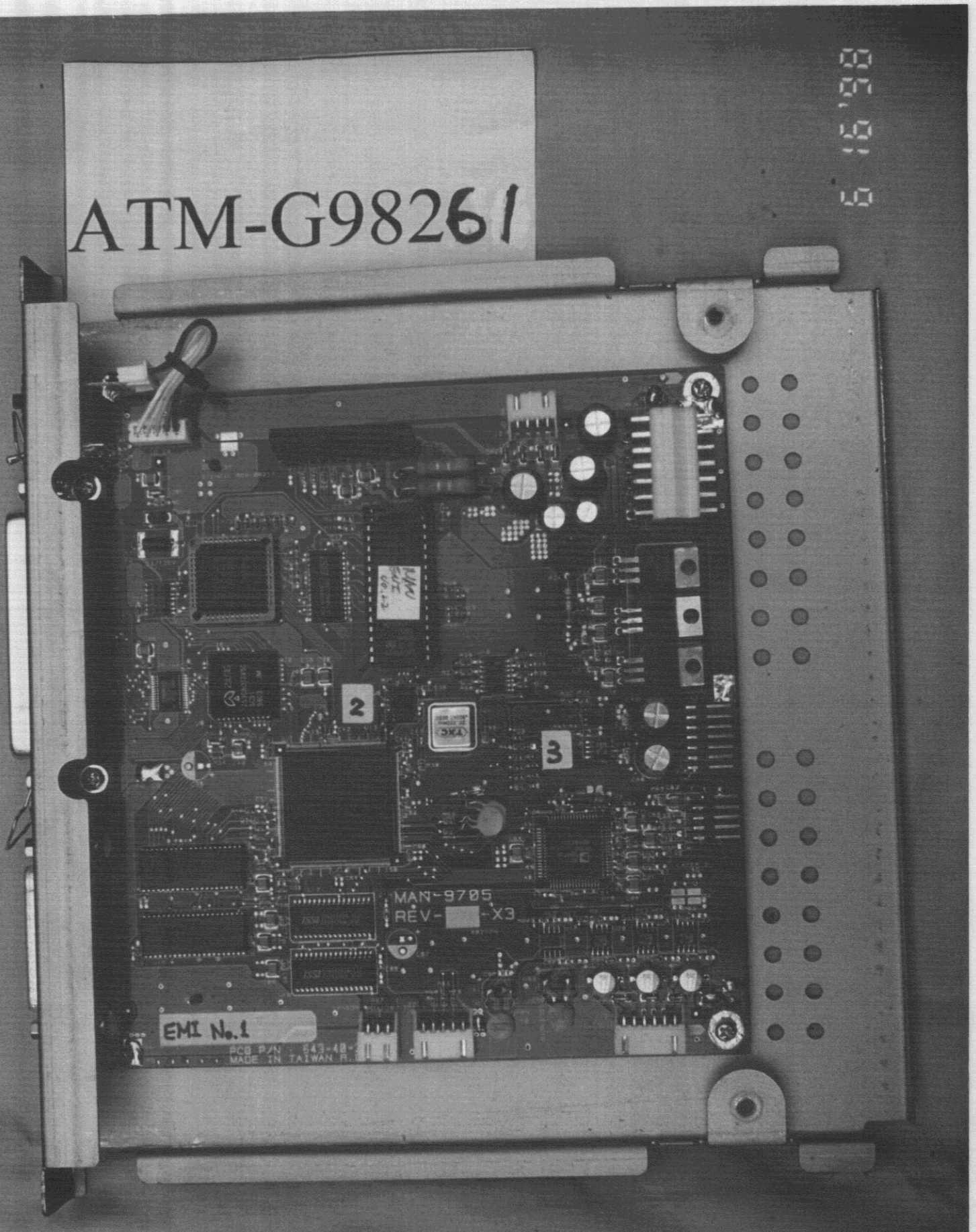
Figure 9 Main Board (Component Side) w/ Metal Cover
