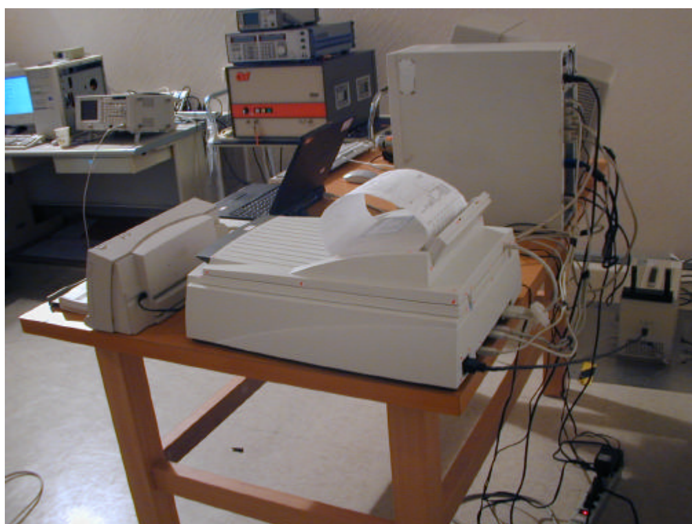
Back View of Conducted Test (Mode 2 —Link PC, W/1394 Cable (1.5M)
