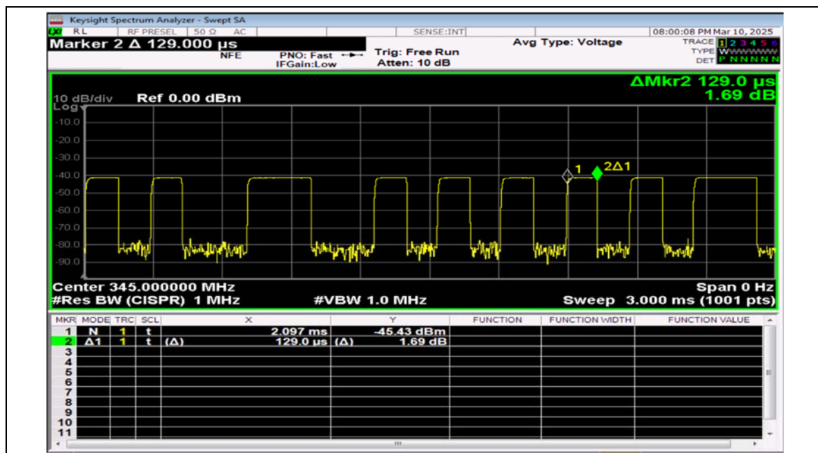
(Duty cycle)
