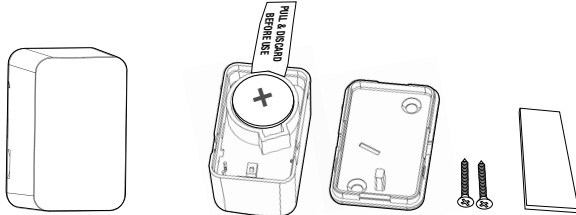
Figure 1. TILT100 Sensor
