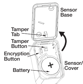
Figure 6. Snap Sensor/Cover onto Sensor Base
