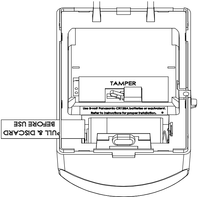
BATTERY LABEL LOCATION DETAIL SCALE 2:1 (BACK COVER REMOVED FOR CLARITY)
