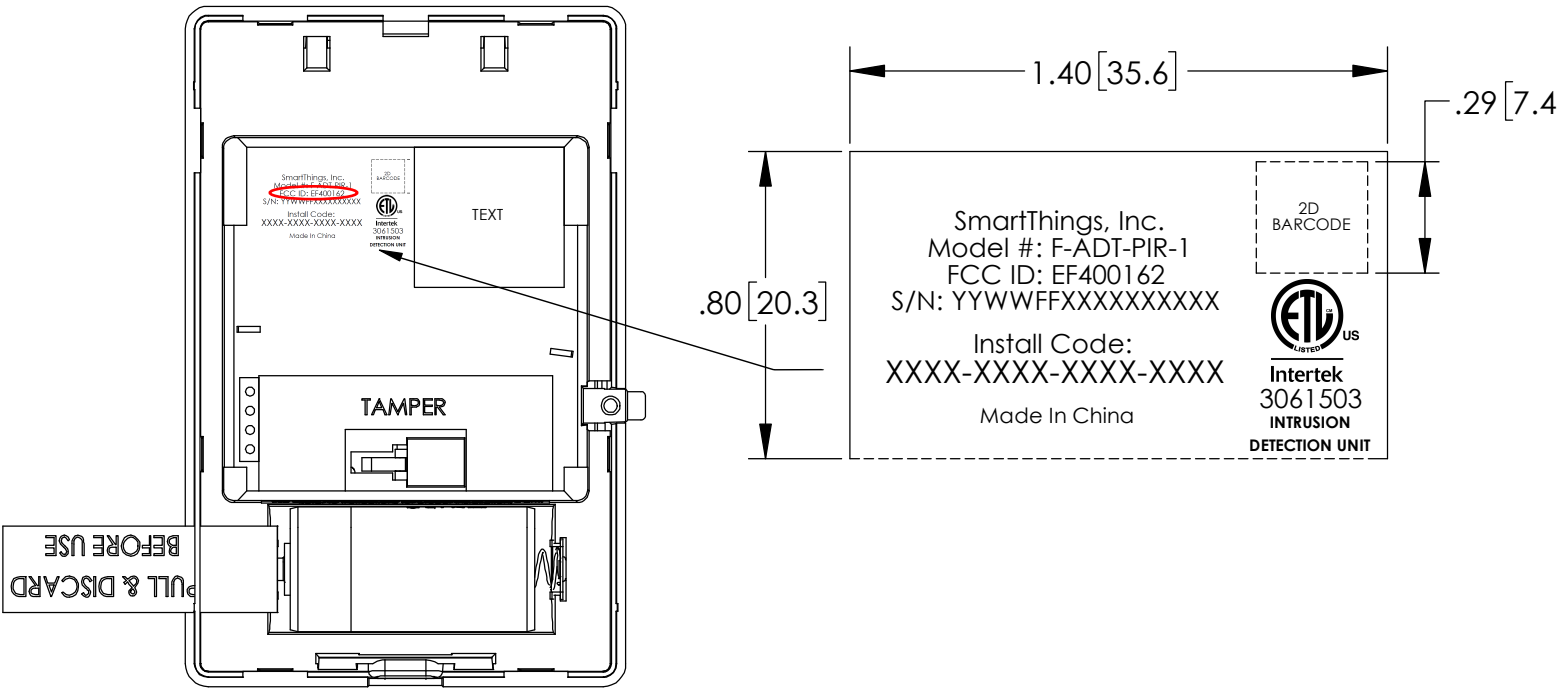
LABEL LOCATION DETAIL SCALE 2:1 (BACK COVER REMOVED FOR CLARITY)
