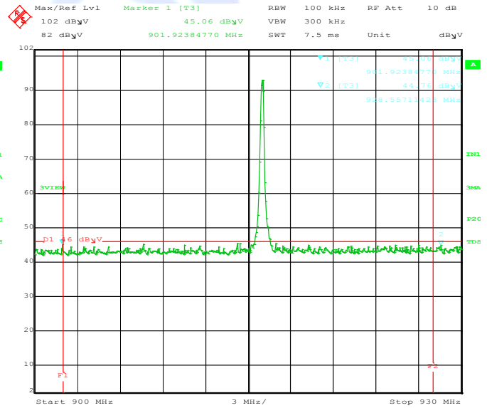
Comment A: Band Edge 916MHz Vertical Date: 17.MAY.2016 13:10:43
