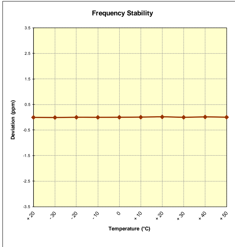
Figure 6-9. Frequency Stability Graph (PCS CDMA Mode – Ch. 600)
