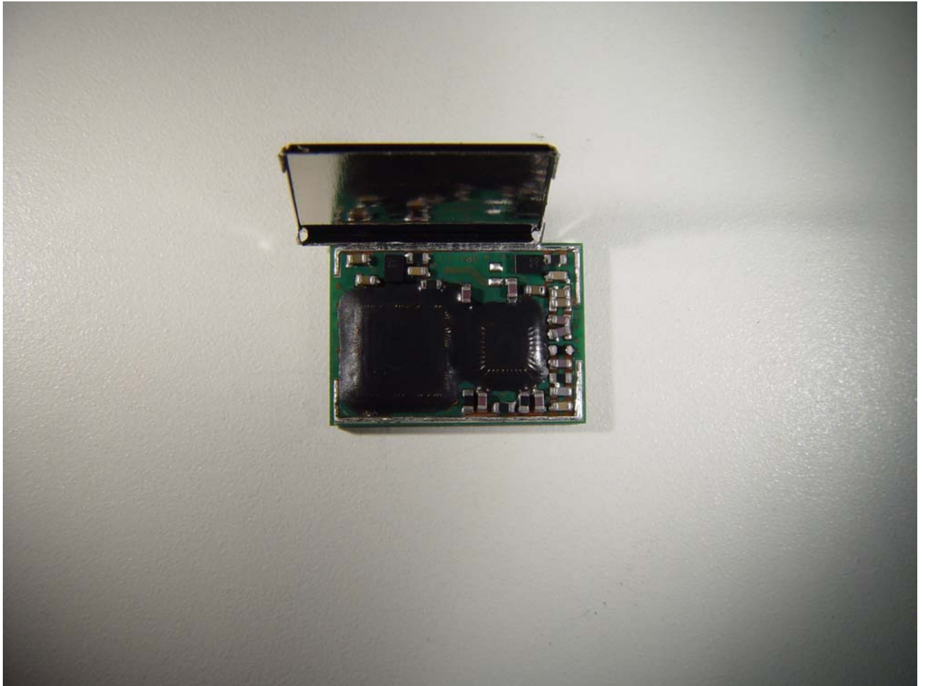
LMX9820A internal photo
