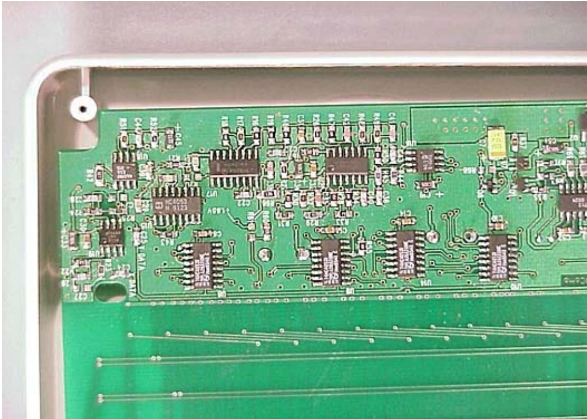
Top of board – section 1
