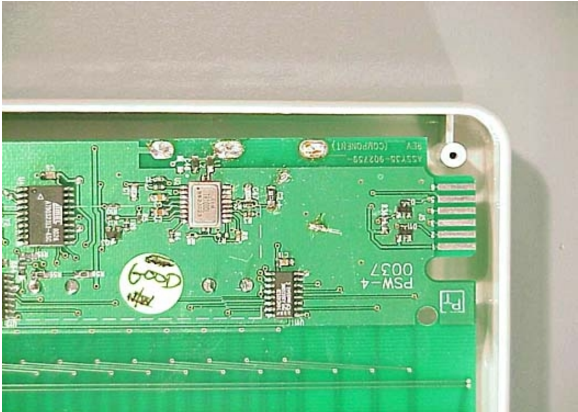
Top of board, section 4
