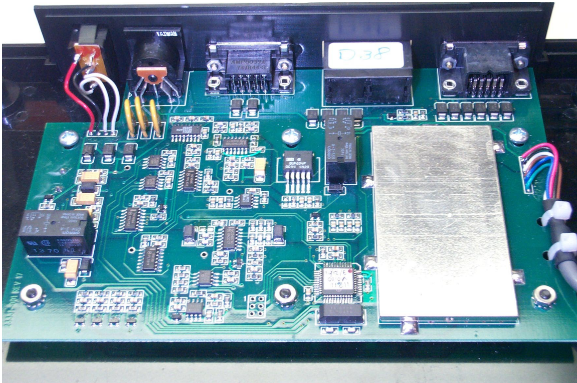
Figure 9.0-1 BDR-1000 Internal View – Control Board
