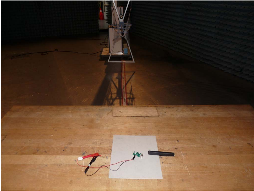
Photo 1: Test setup for radiated measurements (Enclosure, semi-anechoic chamber, 30 MHz to 1 GHz, intentional radiator §15)
