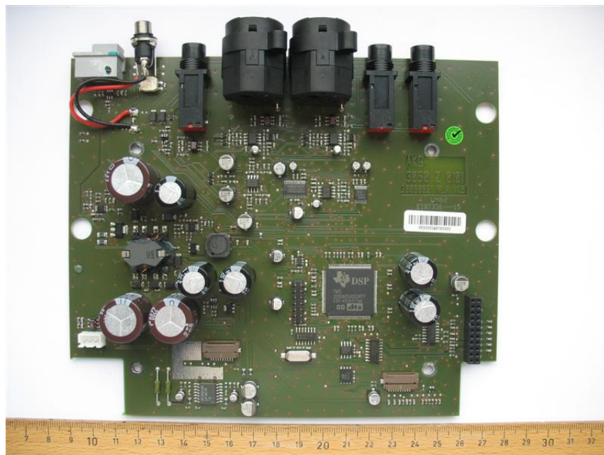
Photo 14: (SST 4 – Transmitter)
