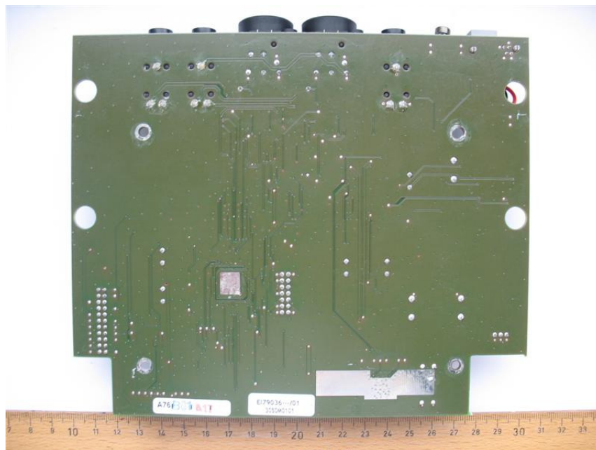
Photo 16: (SST 4 – Transmitter)
