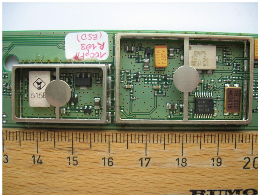
Photo 12: (SST 4 – Transmitter)
