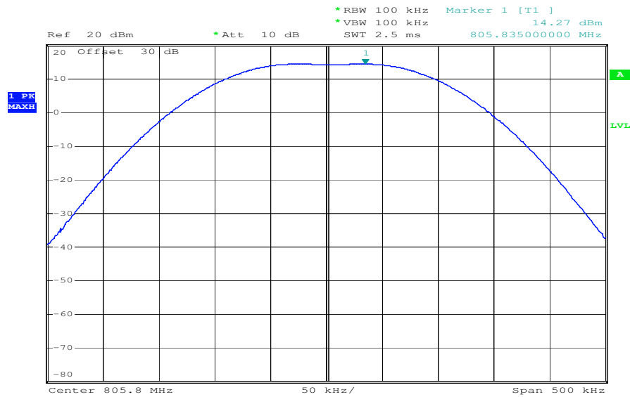
Plot 5: Output Power Transmitter
