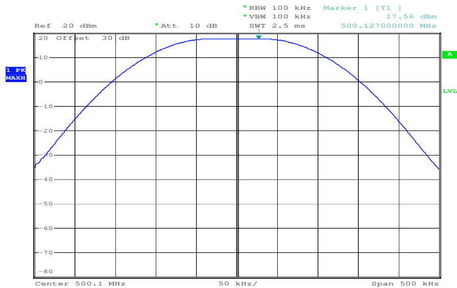
Plot 1: Output Power Transmitter
