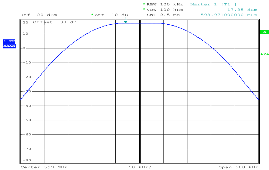
Plot 3: Output Power Transmitter
