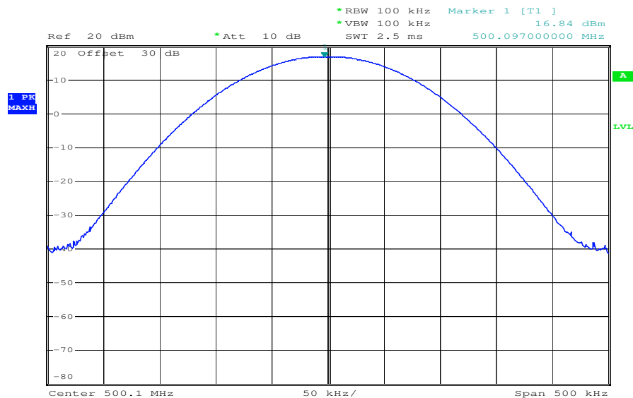
Plot 2: Output Power Antenna Combiner
