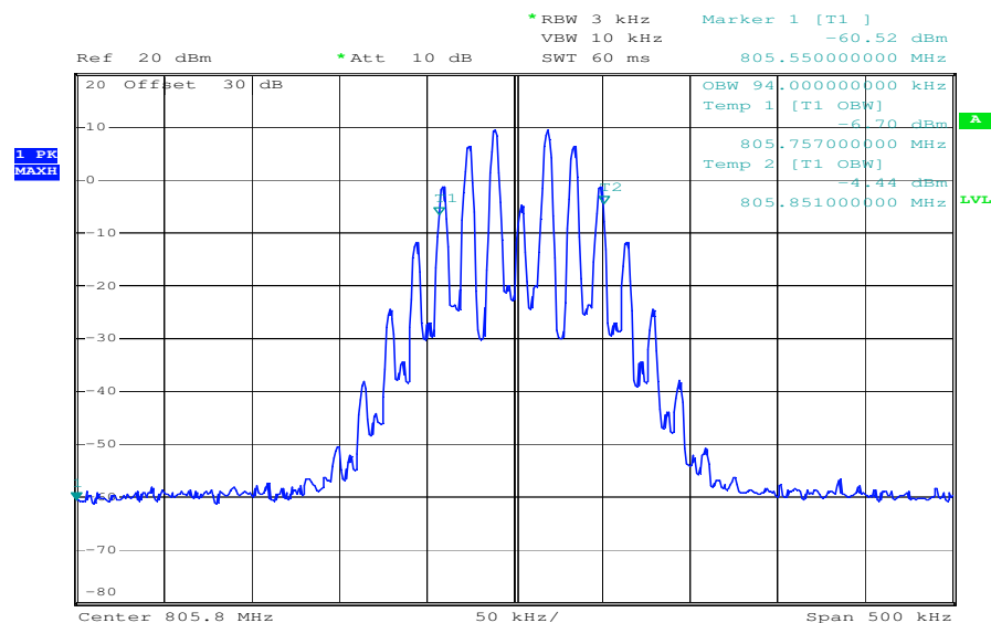
Plot 6: 805.8 MHz – Output Antenna Combiner
