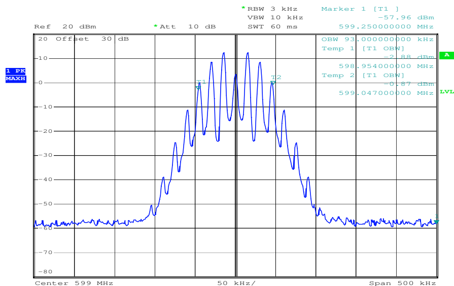
Plot 4: 599 MHz – Output Antenna Combiner
