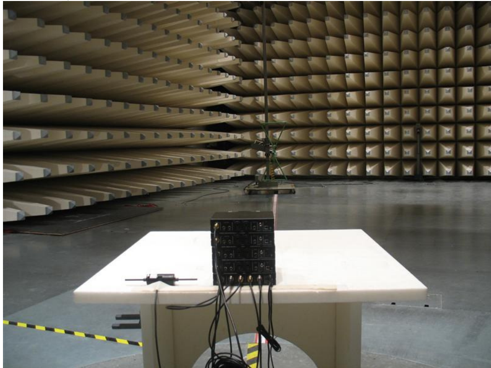
Photo 1: (Radiated Emission)
