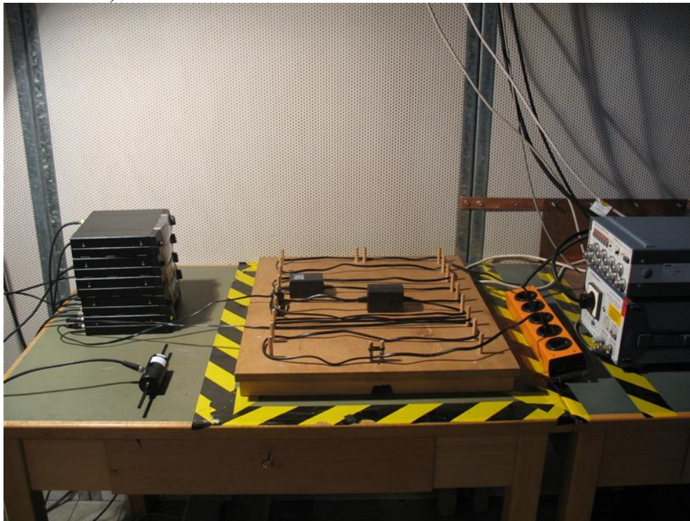
Photo 5: (Conducted Emission)
