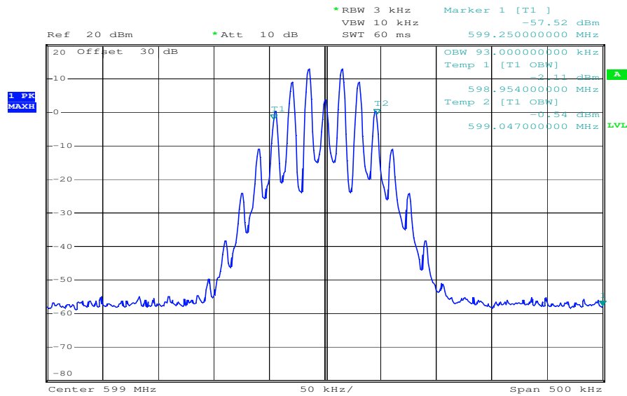
Plot 3: 599 MHz – Output Transmitter
