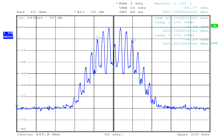
Plot 5: 805.8 MHz – Output Transmitter
