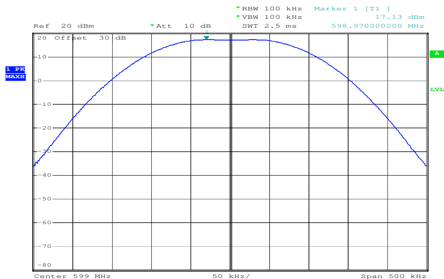
Plot 4: Output Power Antenna Combiner
