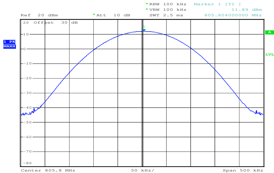
Plot 6: Output Power Antenna Combiner
