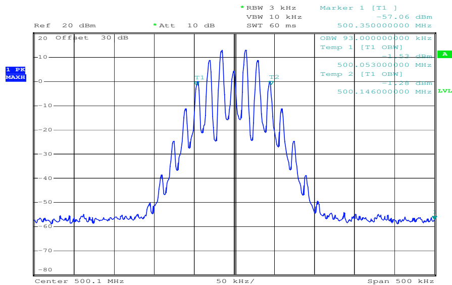
Plot 1: 500.1 MHz – Output Transmitter
