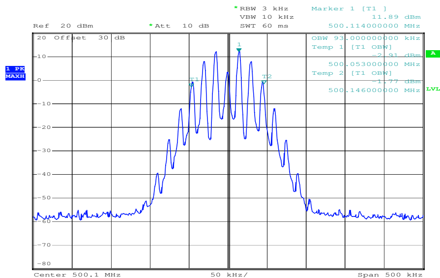
Plot 2: 500.1 MHz – Output Antenna Combiner
