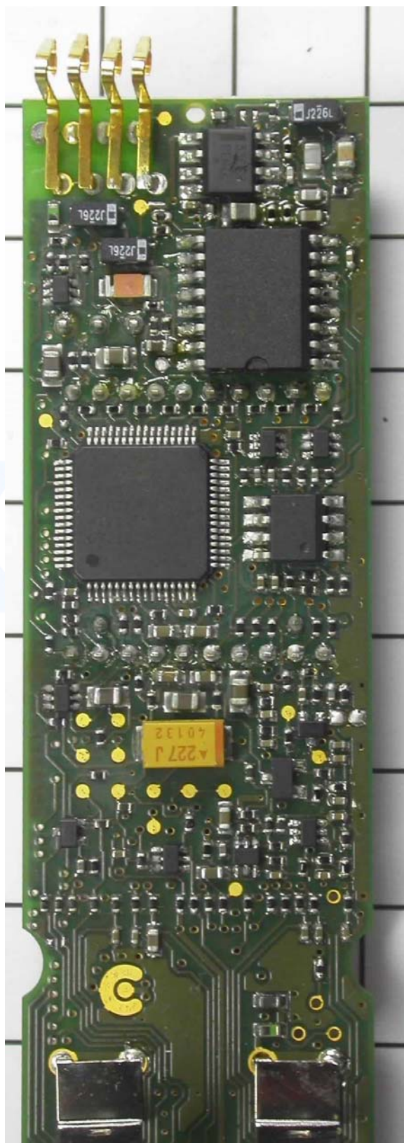
Detailed front view of PCB (top)
