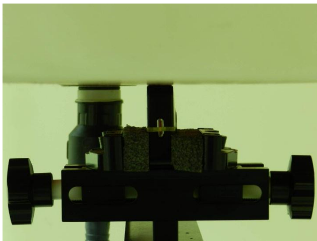
Right Side of the DUT with Phantom 0 cm Gap
