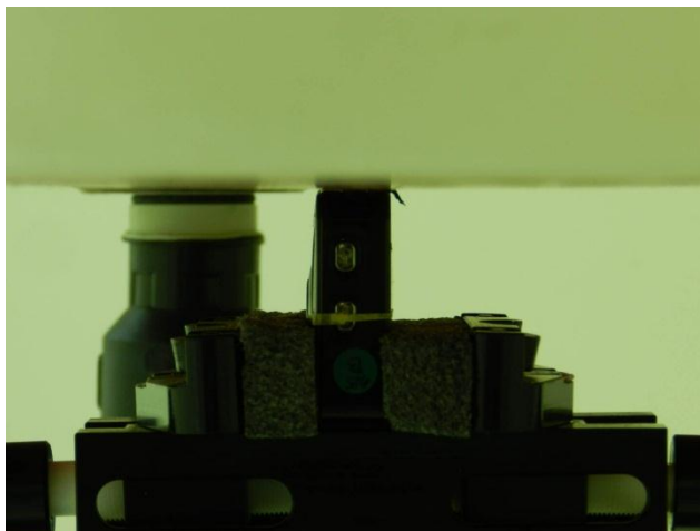
Bottom Side of the DUT with Phantom 0 cm Gap
