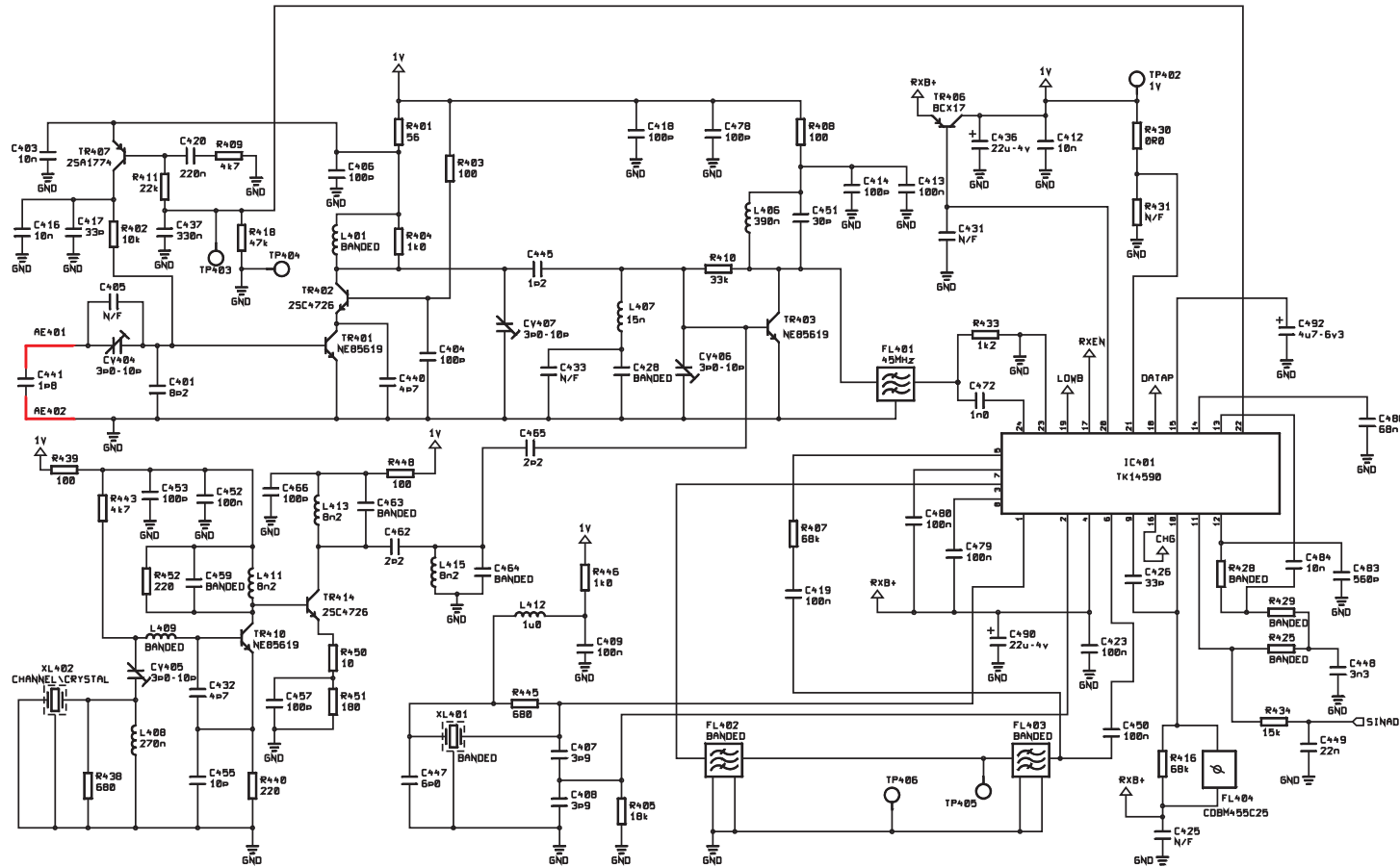
TL853T RADIO CIRCUIT DIAGRAM 2961-5025 ISS 5 SHT 1 OF 2
